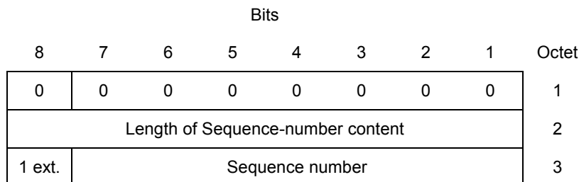
FIGURE 20/G.964
