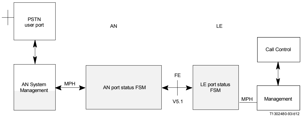
FIGURE 32/G.964 Port operation and maintenance functional model
