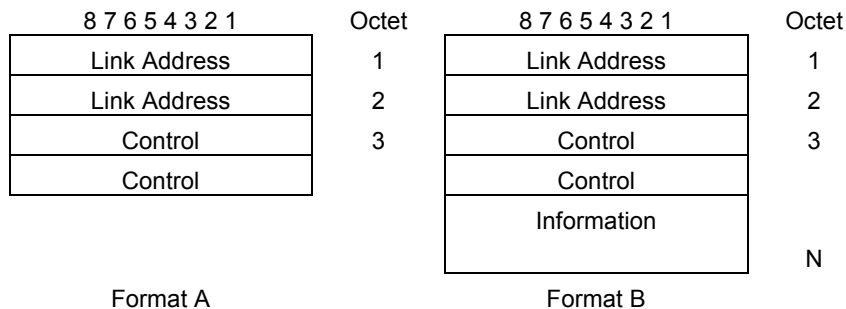
FIGURE 9/G.964
