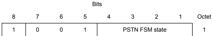
FIGURE 17/G.964 State information element
