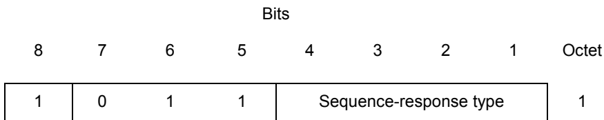
FIGURE 19/G.964
