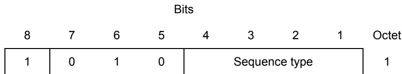
FIGURE 18/G.964
