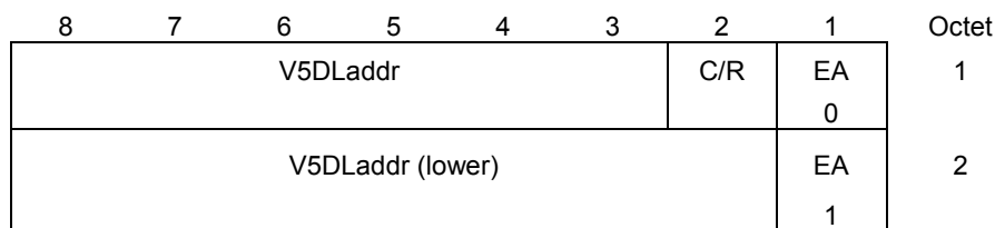
FIGURE 10/G.964
