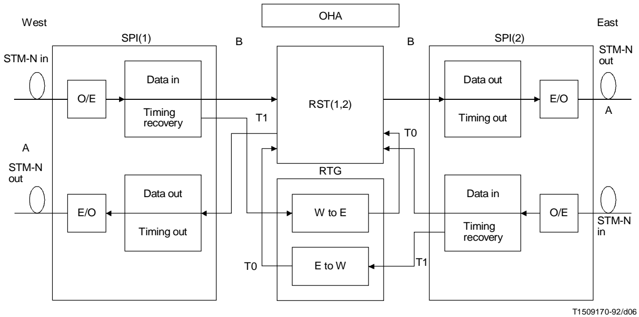
FIGURE 9-1/G.958 Description of the regenerator timing functions
