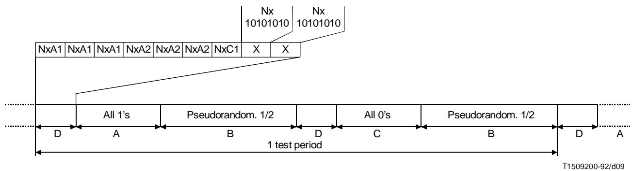
FIGURE I.1/G.958 STM-N pattern dependence test sequence
