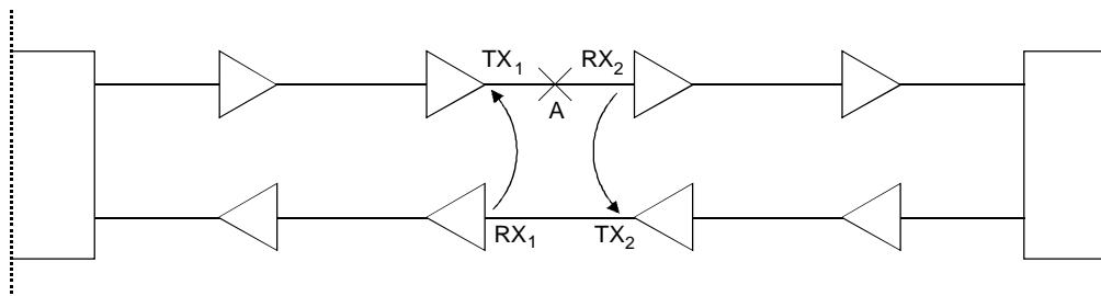
FIGURE II.1/G.958 Description of ALS capability in case of cable break
