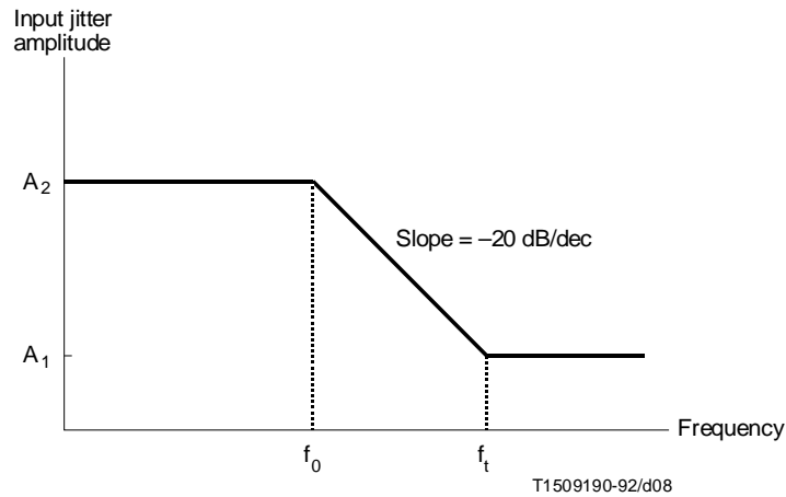
FIGURE 9-3/G.958 Jitter tolerance mask
