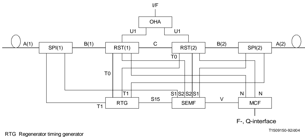
FIGURE 8-2/G.958 Regenerator model
