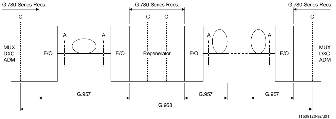
FIGURE 5-1/G.958 Inter-office link
