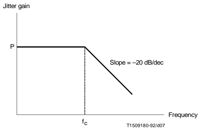
FIGURE 9-2/G.958 Jitter transfer
