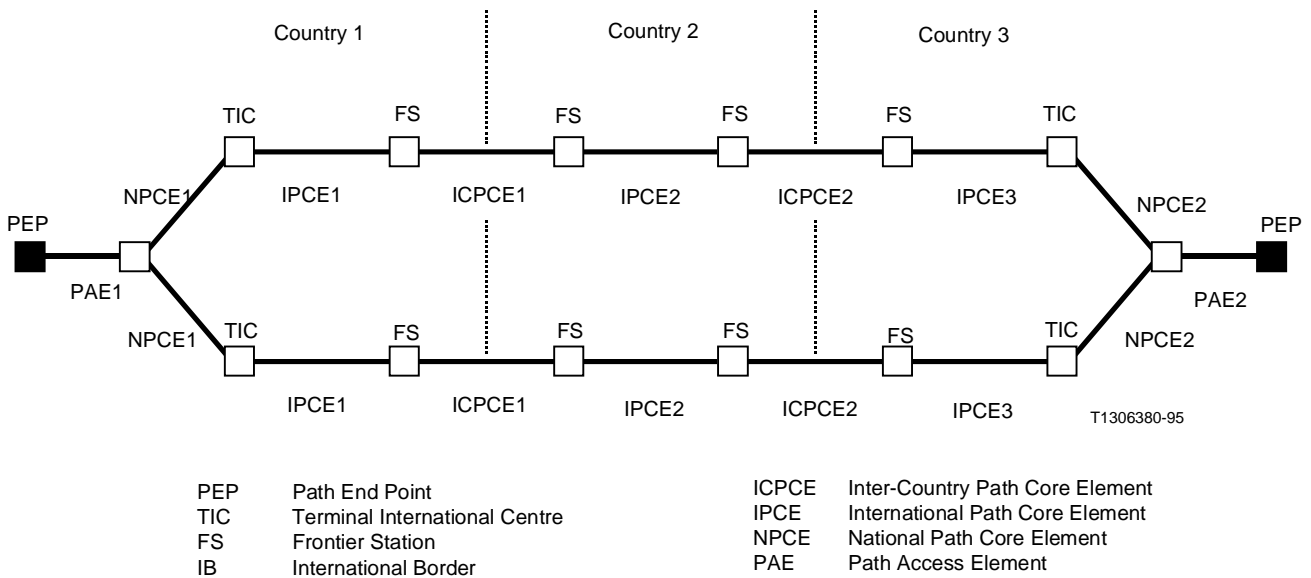
FIGURE A.3/G.827
