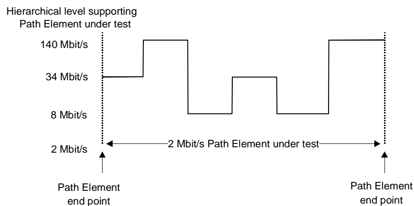
FIGURE B.1/G.827
