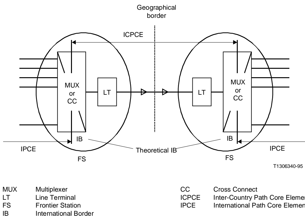
FIGURE 3/G.827
