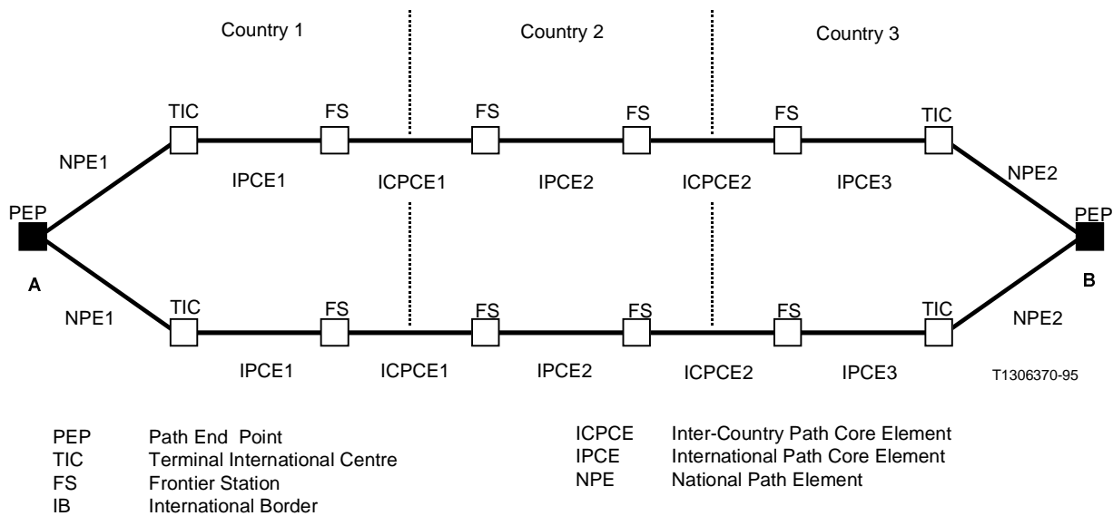
FIGURE A.2/G.827
