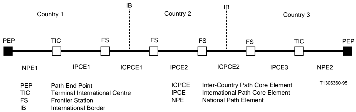
FIGURE A.1/G.827
