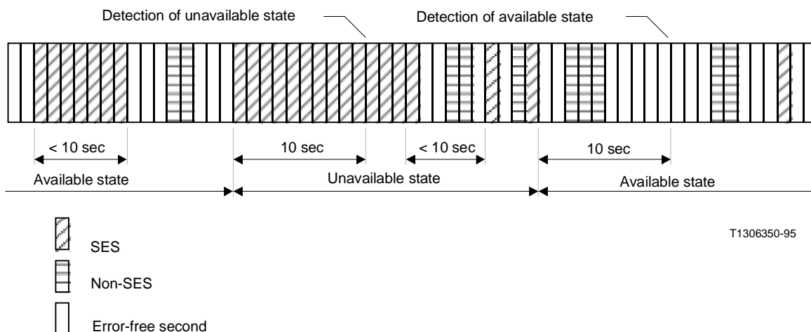
FIGURE 4/G.827
