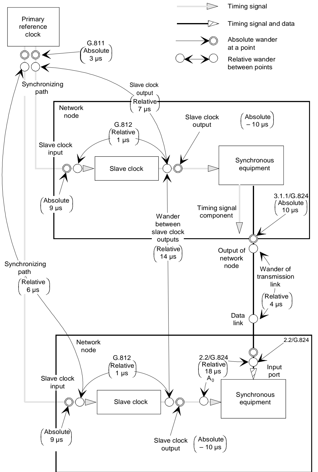
FIGURE A.1/G.824 Wander reference model
