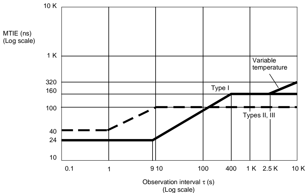
Figure 1/G.812 – Wander generation (MTIE)
