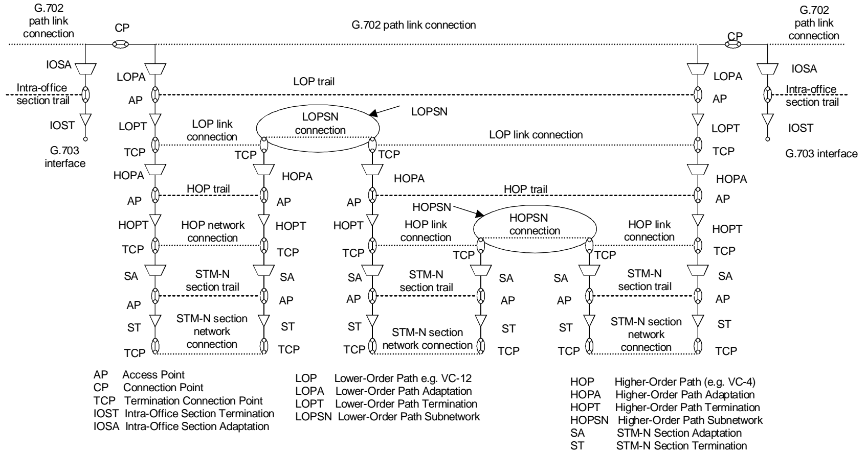
FIGURE 14/G.805
