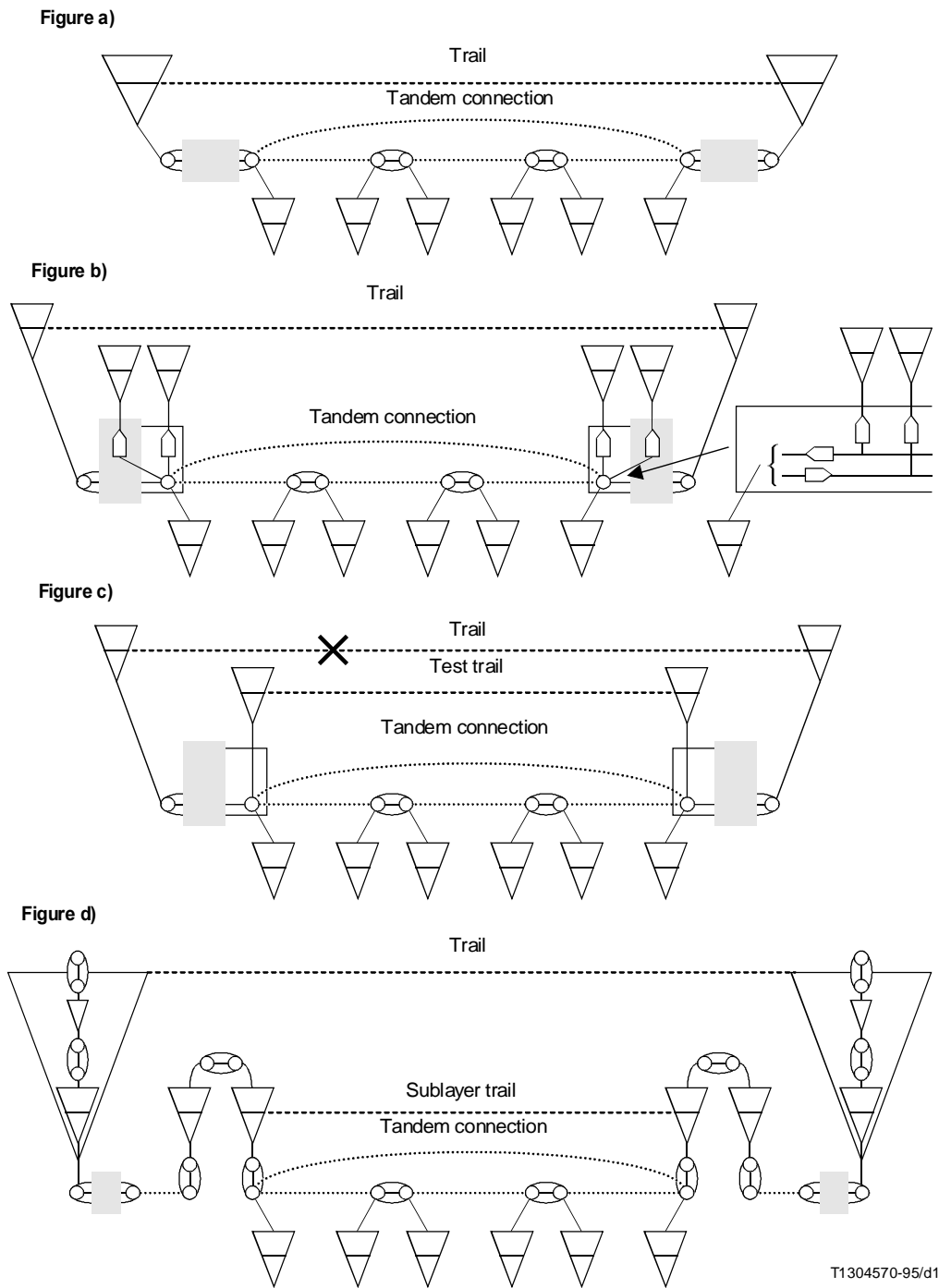
FIGURE 12/G.805 Connection monitoring
