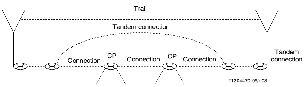
FIGURE 2/G.805 (concluded) Other diagrammatic conventions
