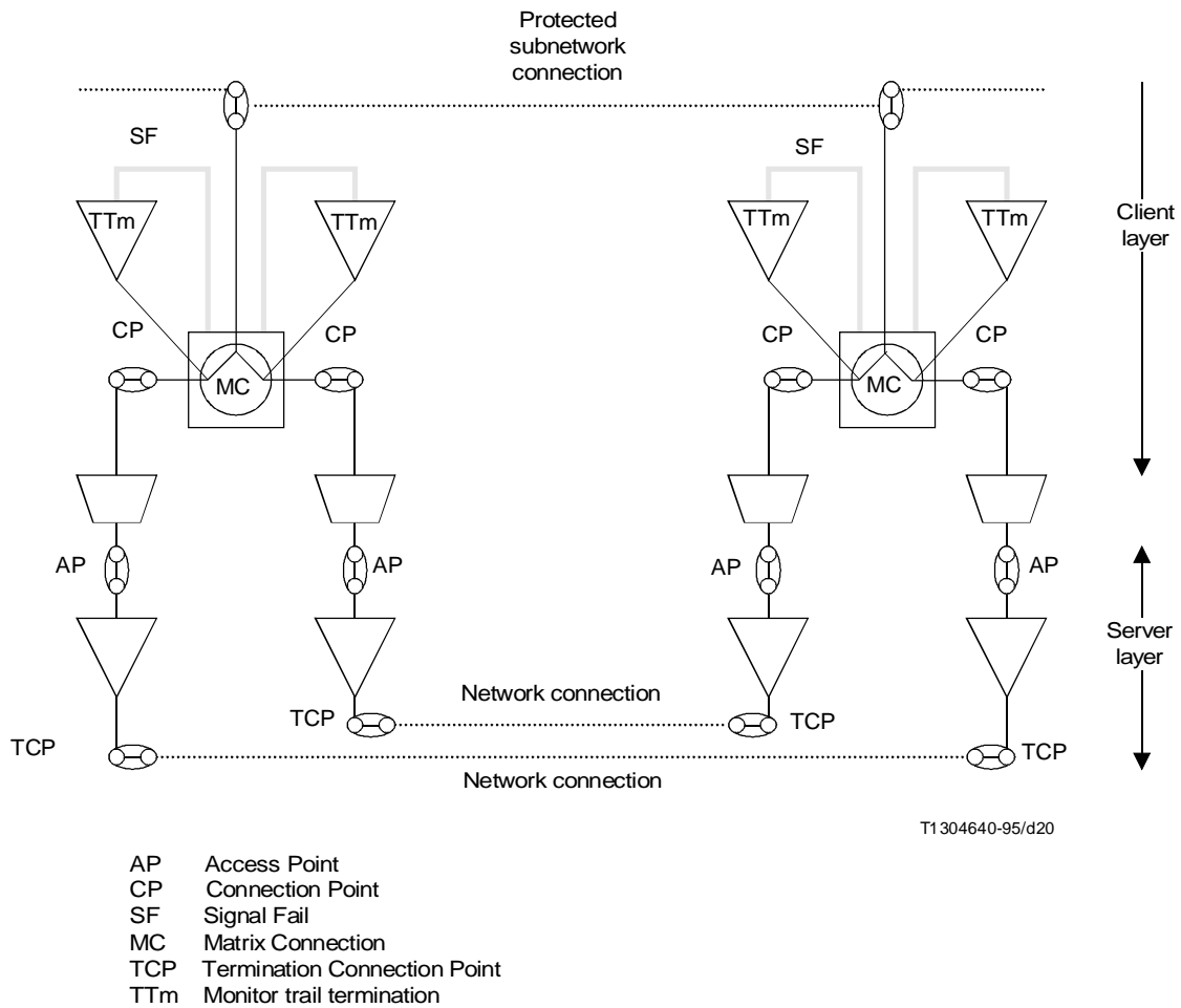
FIGURE 19/G.805 Subnetwork connection protection using non-intrusive monitoring
