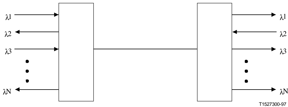
Figure VII.2/G.692 – Bidirectional WDM
