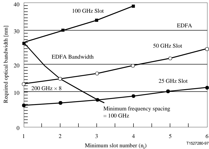
Figure V.3/G.692 – Required optical bandwidth
