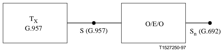
Figure 2/G.692 – Possible implementation of a G.692 transmitter using a G.957 compliant transmitter and a transponder
