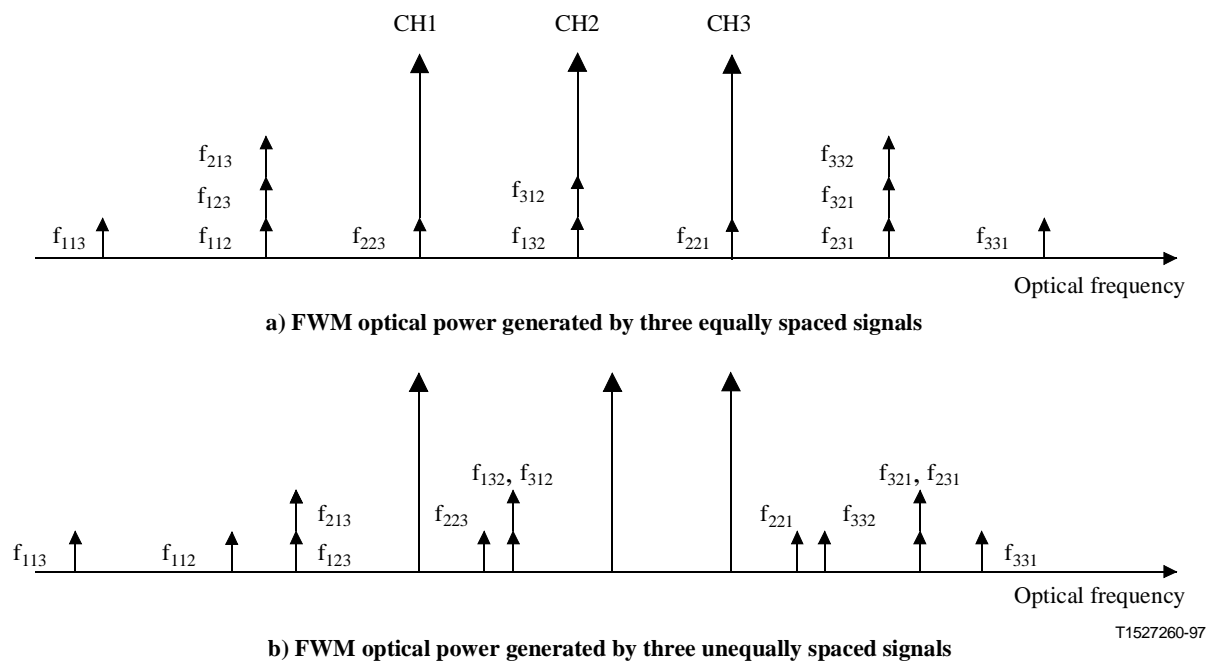
Figure V.1/G.692 – An Example of signal frequencies and resultant FWM optical powers
