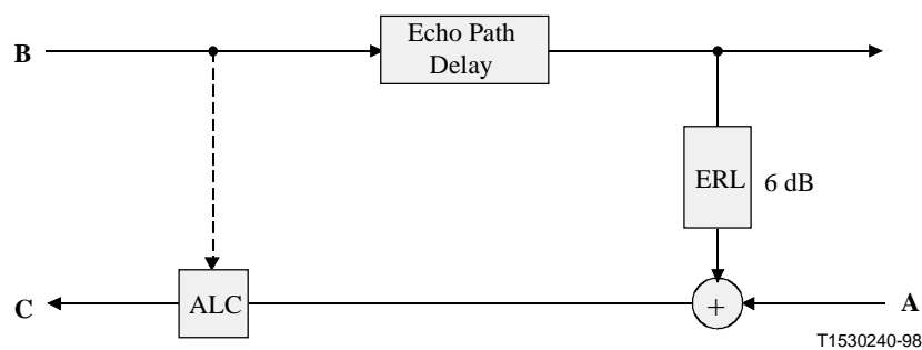
Figure 2/G.169 – Circuit configuration for "Test A" – ALC echo robustness for connections without echo control
