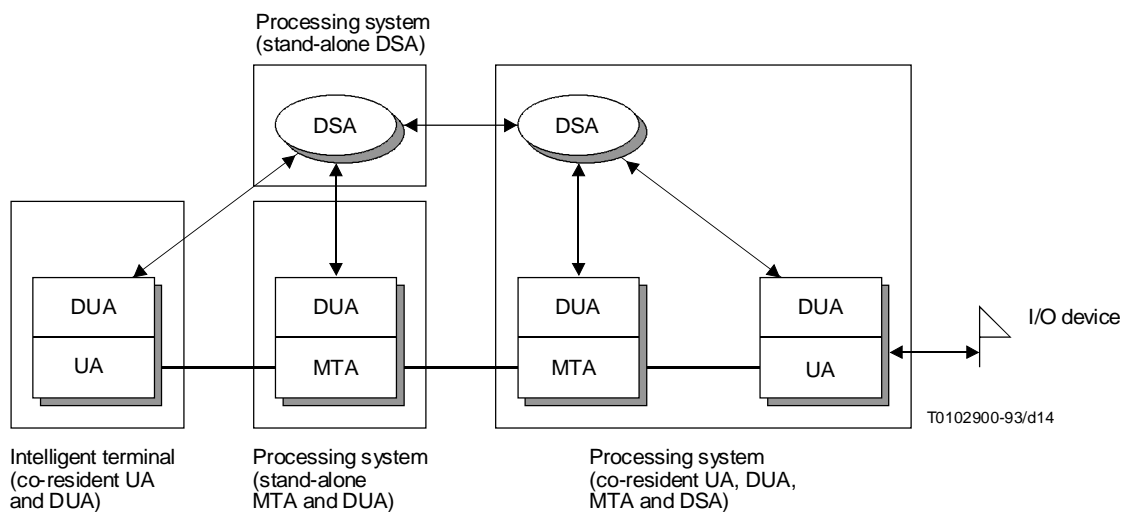
FIGURE 14/F.400 Physical configurations for MHS-directory interworking
