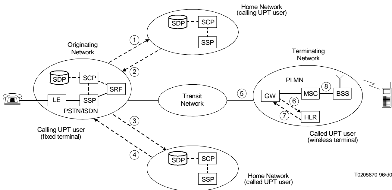
Case b): Called UPT user registered via a wireless terminal
