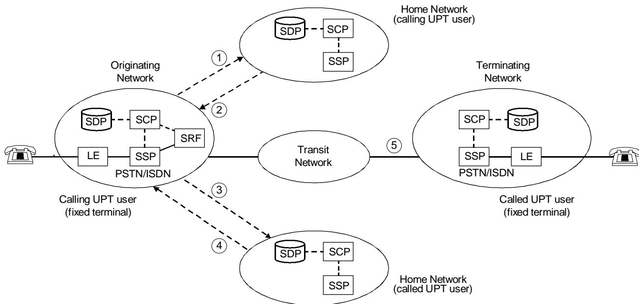
Case a): Called UPT user registered via a fixed terminal
