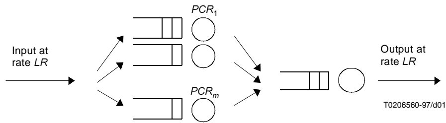
Figure 6-1/E.736 – Conceptual spacer for m peak rate allocated connections ( \sum PCR_i \leq LR )
