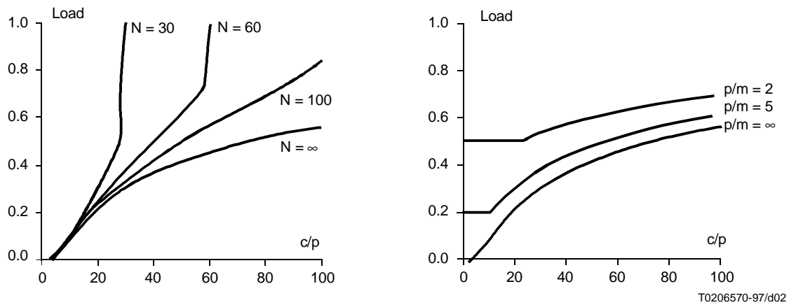
Figure 7-1/E.736 – Achievable load against link to peak ratio ( c/p )
