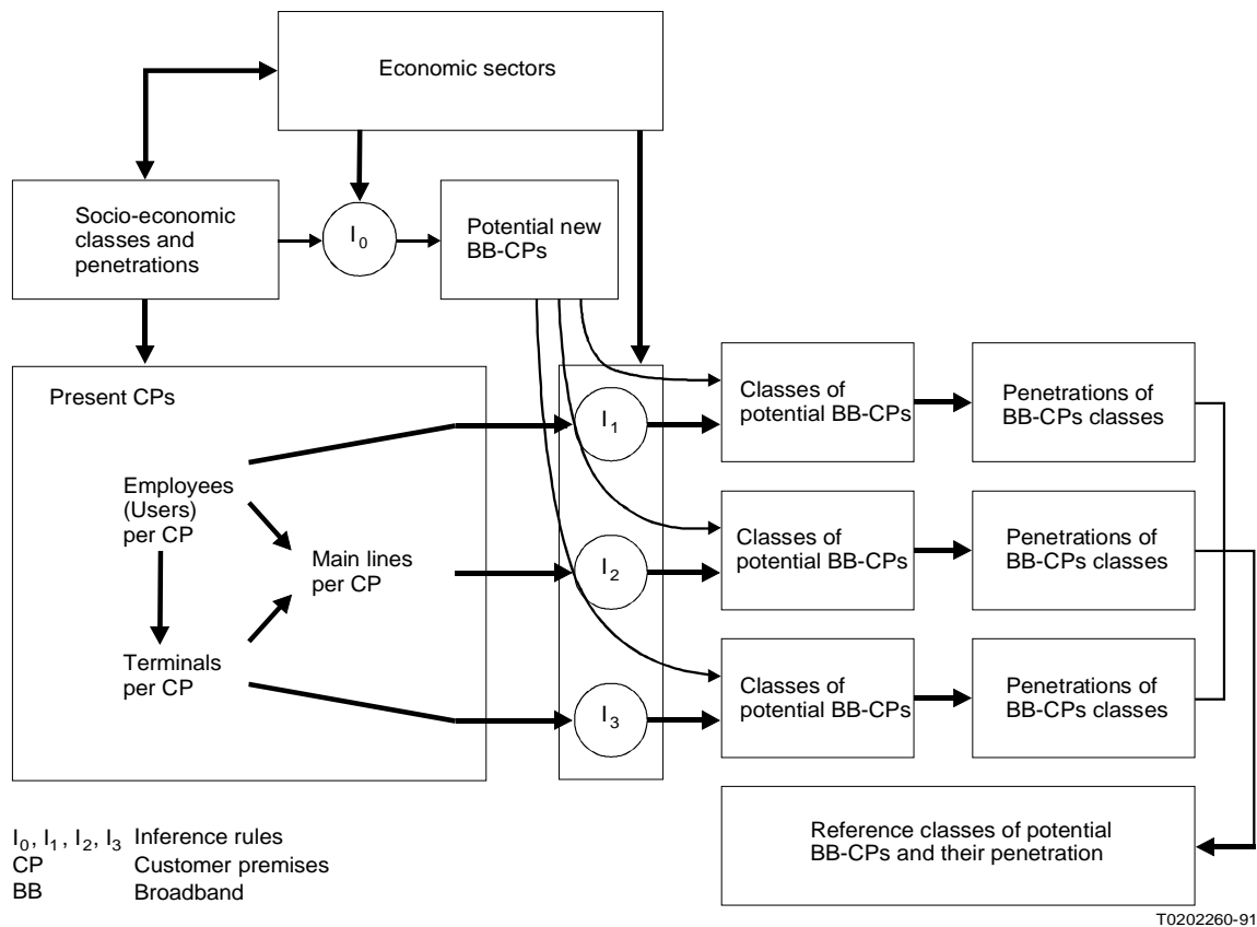
FIGURE 4/E.508 Example of sectorial-econometric forecasting
