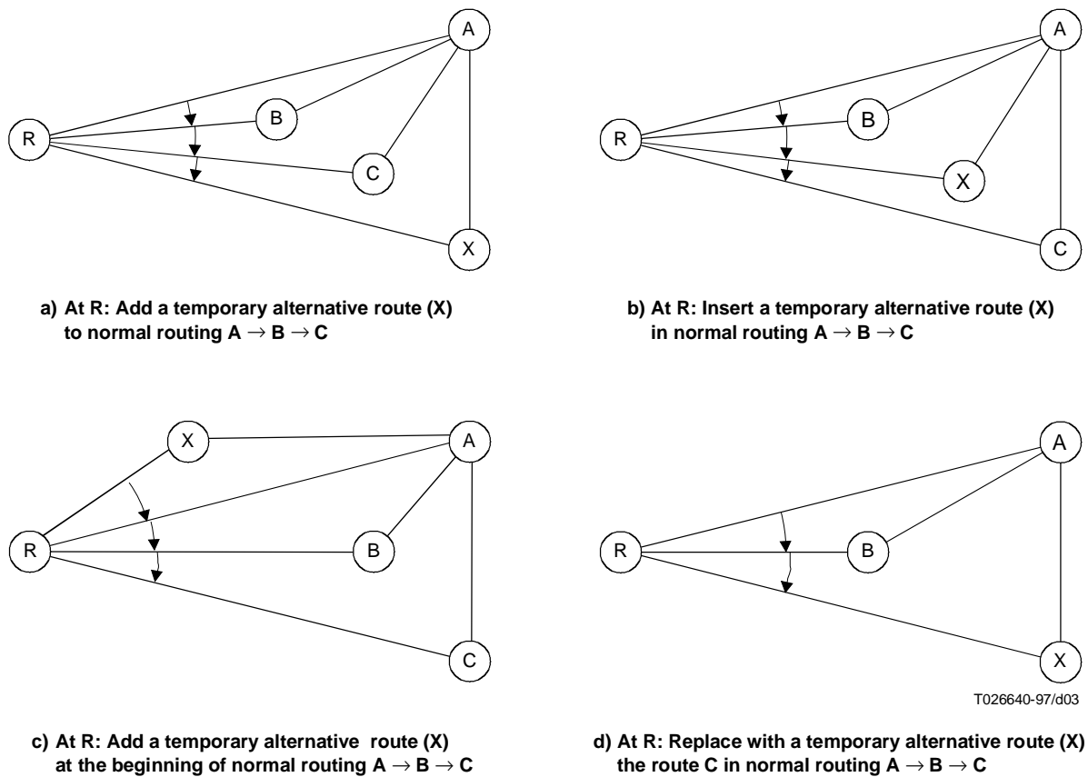
Figure 3/E.412 – Examples of temporary alternative routing
