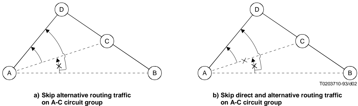
Figure 2/E.412 – Examples of skip
