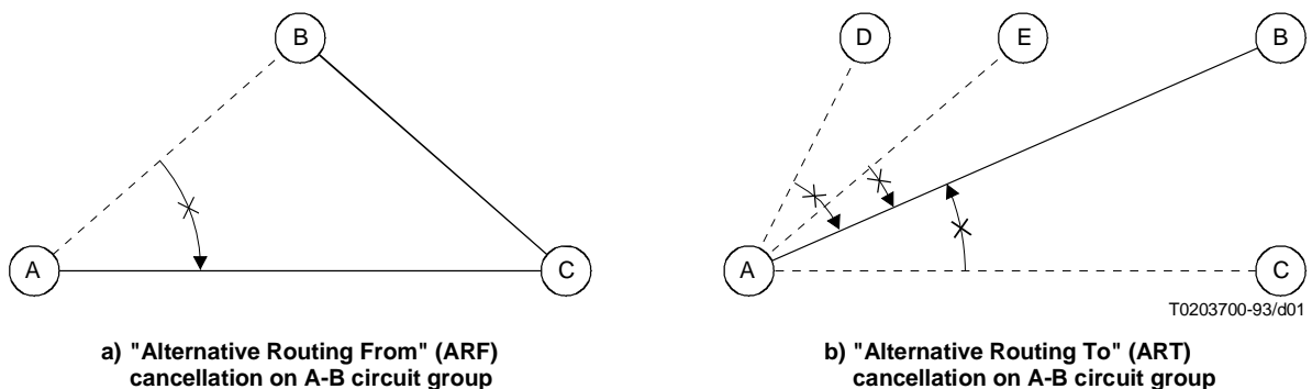
Figure 1/E.412 – Examples of alternative routing cancellation
