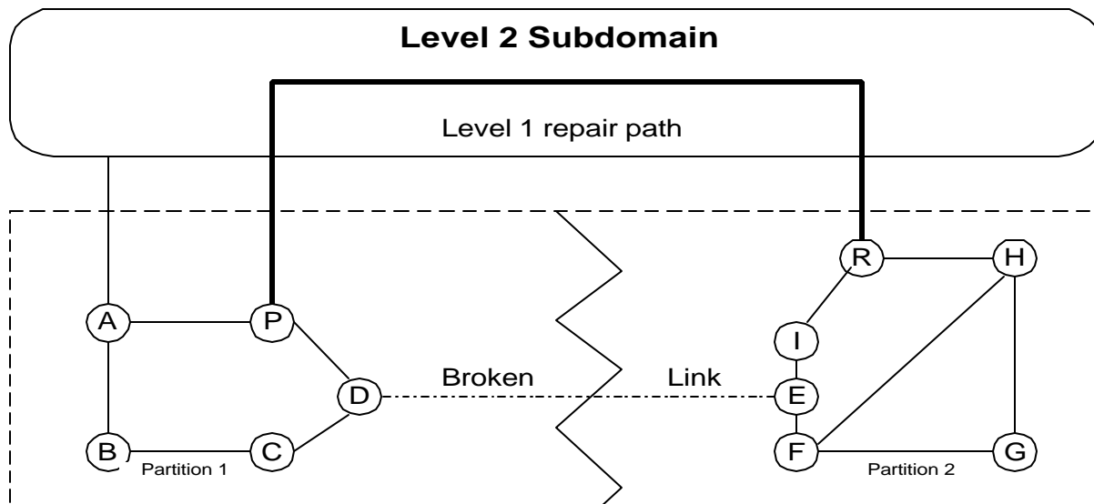
Figure 5 - Repair of partitioned level 1 area
