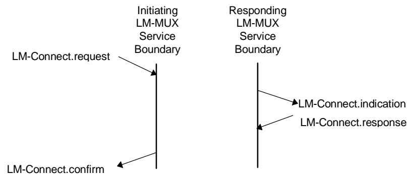
Figure 8. Accepted Connection
