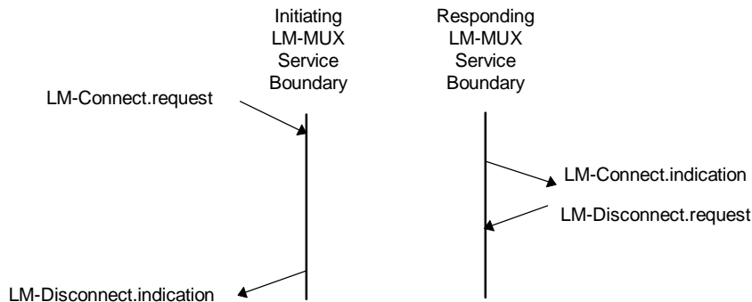
Figure 10. Rejected Connection
