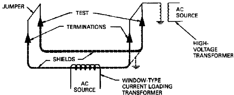
Figure 2—Single-phase terminations
