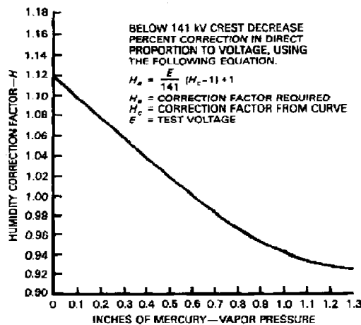
Figure 1—Humidity correction factor, 1.2 \times 50 \mu\text{s} impulse
