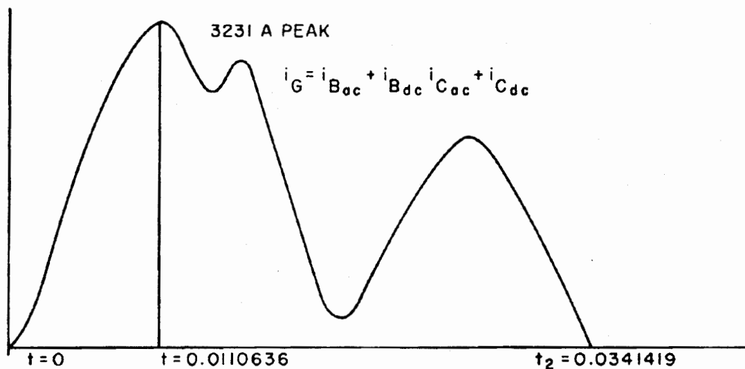
Figure 24—Total current for an evolving fault
