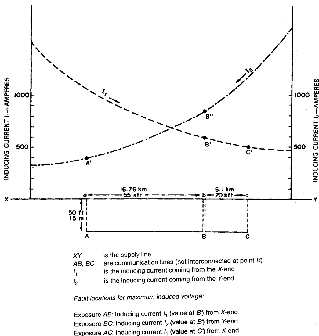
Figure 39—Double-ended supply system feed and inductive exposures for Example 3
