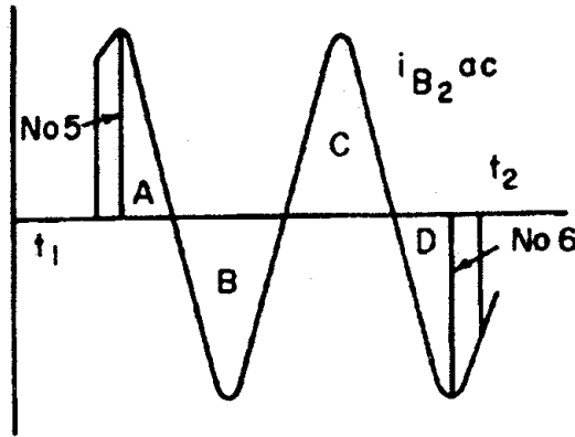
Figure 21—Determination of Areas No. 5 and No. 6 for the second phase B current
