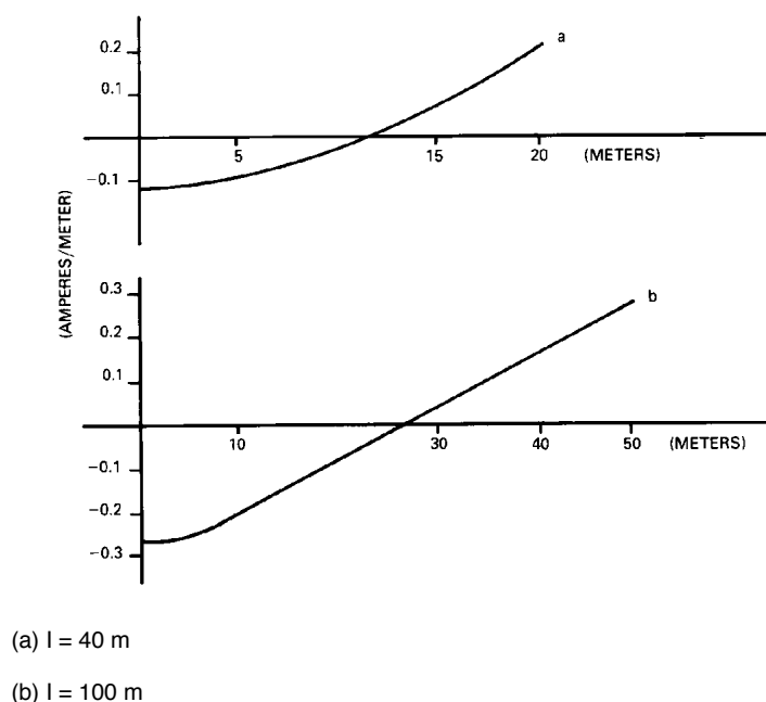
Figure 48—Approximate value of the current absorbed and discharged per length by the conductor metallic sheath of cables subject to interference
