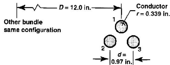
Figure C.4—Battery cable configuration
