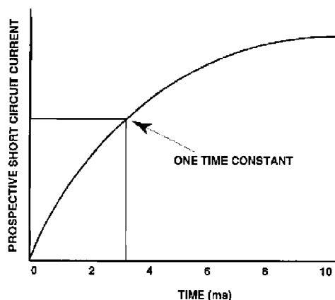
Figure B.2—Short-circuit current rise as a factor of time constant
