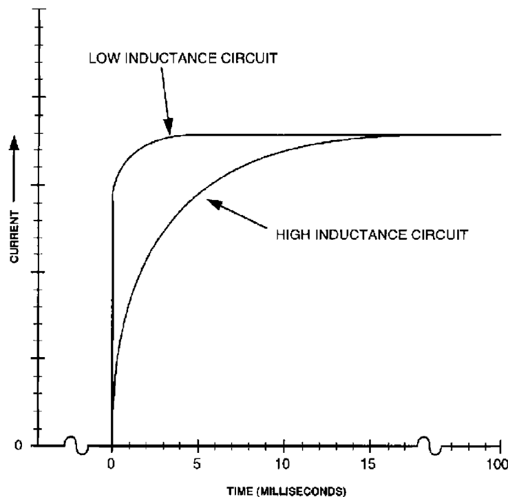
Figure 2—Lead-acid battery typical initial current characteristic during short circuit
