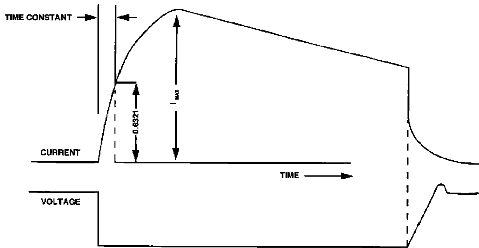
Figure 5—Time constant for dc circuits a
