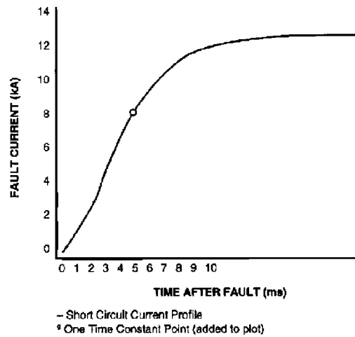
Figure C.2—Battery short-circuit test
