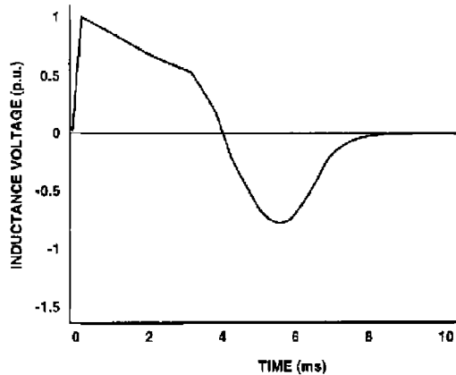
Figure B.3—Circuit inductive voltage
