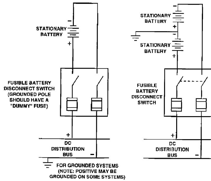
Figure 17—Typical fusible battery disconnect switch schematics— 2-pole switches
