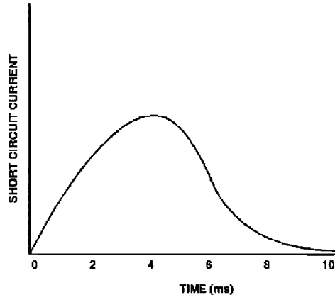
Figure B.4—Short-circuit current interrupted by protective device
