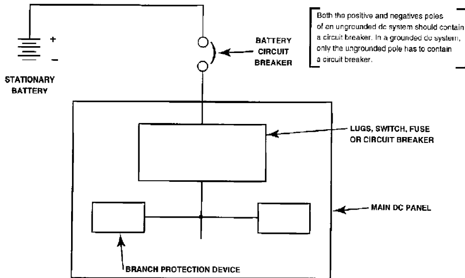
Figure 14—Circuit breakers between the battery terminals and main dc panel
