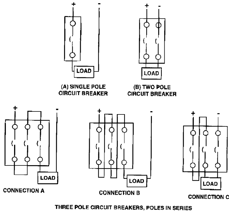
Figure 9—Common circuit breaker dc connections
