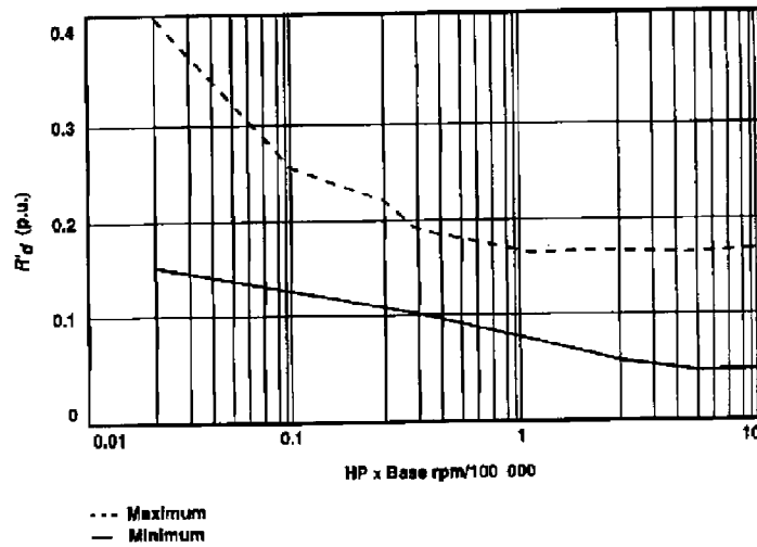
Figure C.3—Transient resistance of dc motor armature circuit
