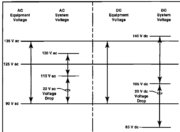
Figure 11—AC versus dc voltage regulation
