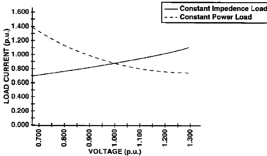
Figure 12—Voltage effects on current
