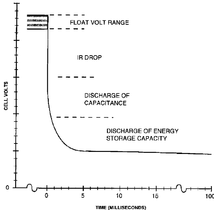
Figure 1—Lead-acid battery typical initial voltage characteristic during short circuit
