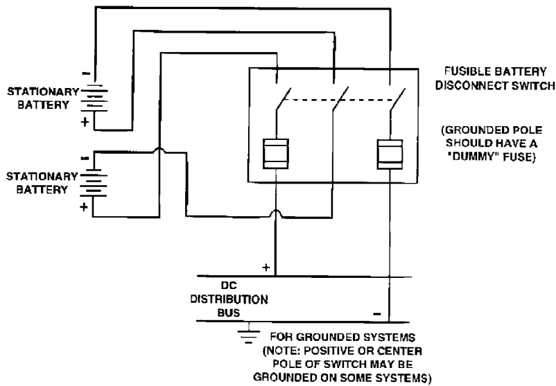
Figure 18—Typical fusible battery disconnect switch schematics— 3-pole switches
