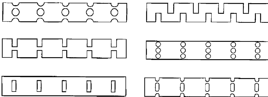
Figure 4—Typical bridges used in fuse link construction
