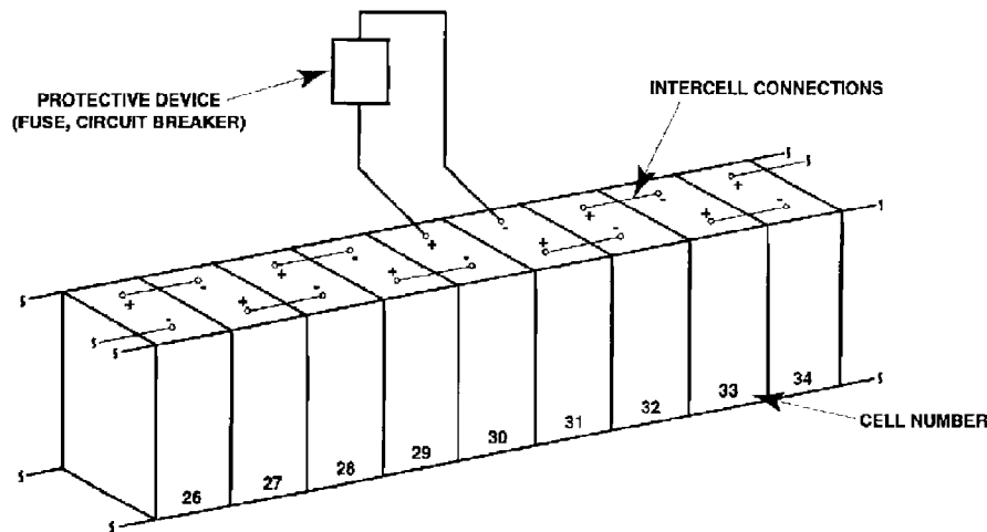
Figure 20—Mid-span protection for a 60-cell stationary battery
