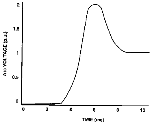
Figure B.5—Voltage applied across protective device
