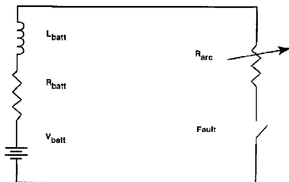
Figure B.1—Schematic of a simple battery system
