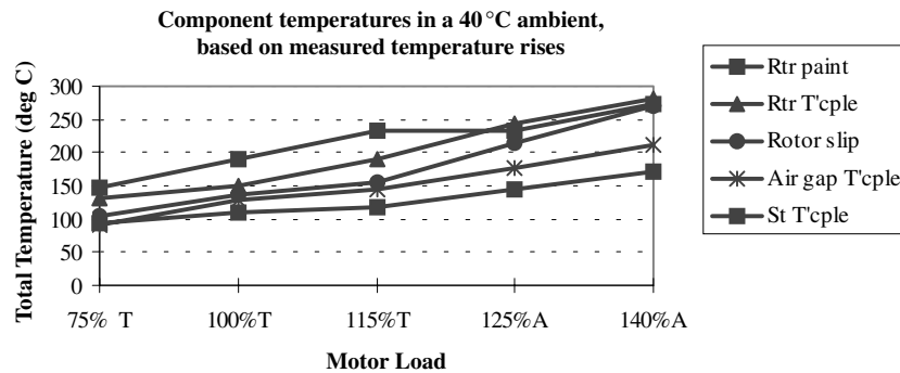
Figure H.2—10 hp four-pole standard efficiency TEFC motor, measured temperature
