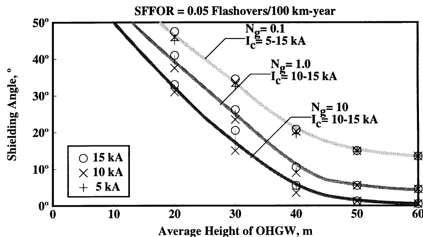
Figure 3—Shielding angles for constant SFFOR using striking distance equations from 5.2 and assuming vertical strokes
