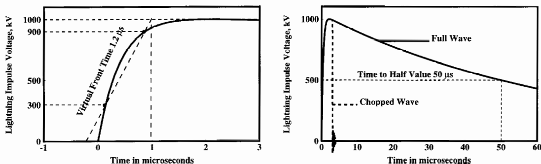
Figure 5—Standard lightning impulse
