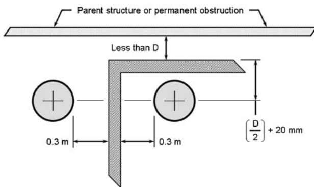
e) Partially accessible corner seam measurements
