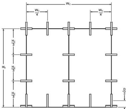
c) Double-panel entry door measurements
