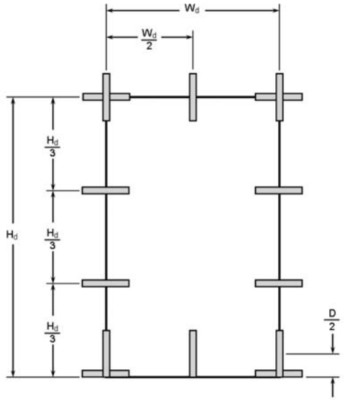
a) Single-panel entry door measurements
