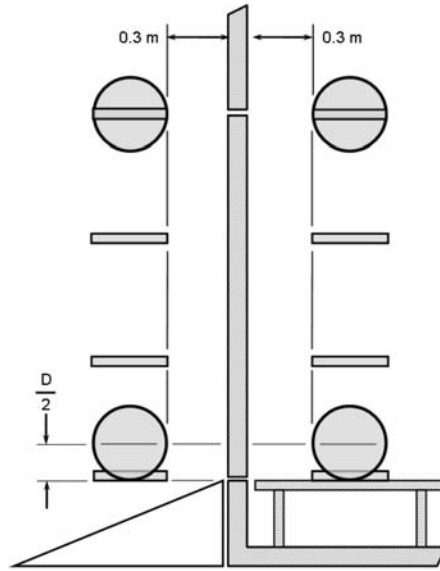
b) Door measurements
