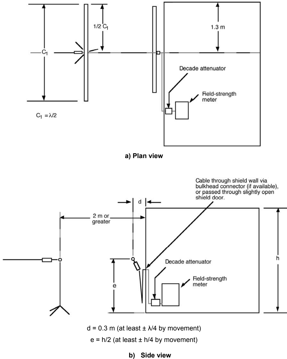
Figure 6—Reference setup for frequencies \leq 1000 \text{ MHz}
