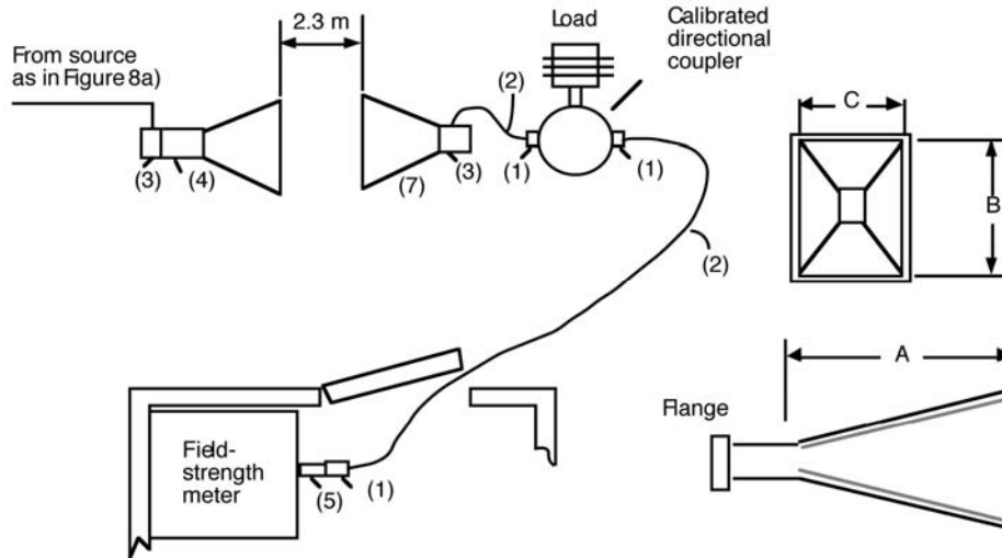
b) Enclosure free-field simulation
