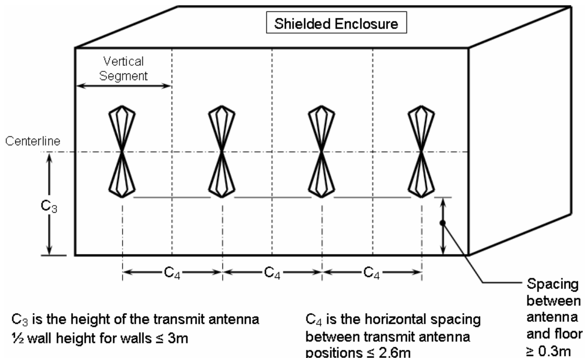
d) Transmitter configuration for measurement setup (vertical antenna orientation), 20 MHz–100 MHz
