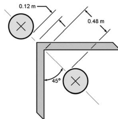
f) Fully accessible corner seam measurements
