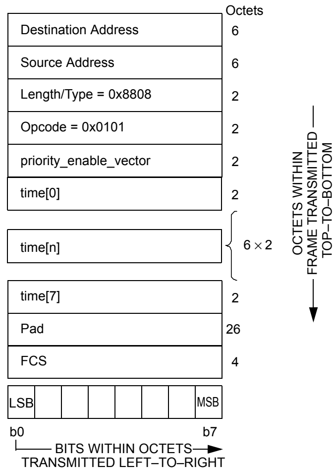
Figure 31D-1—MAC Control EXTENSION Frame
