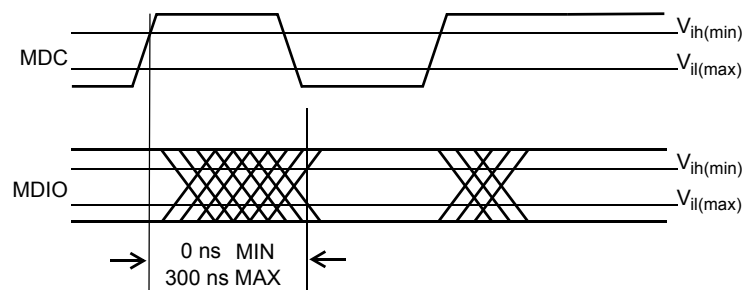
Figure 22-19—MDIO sourced by PHY
