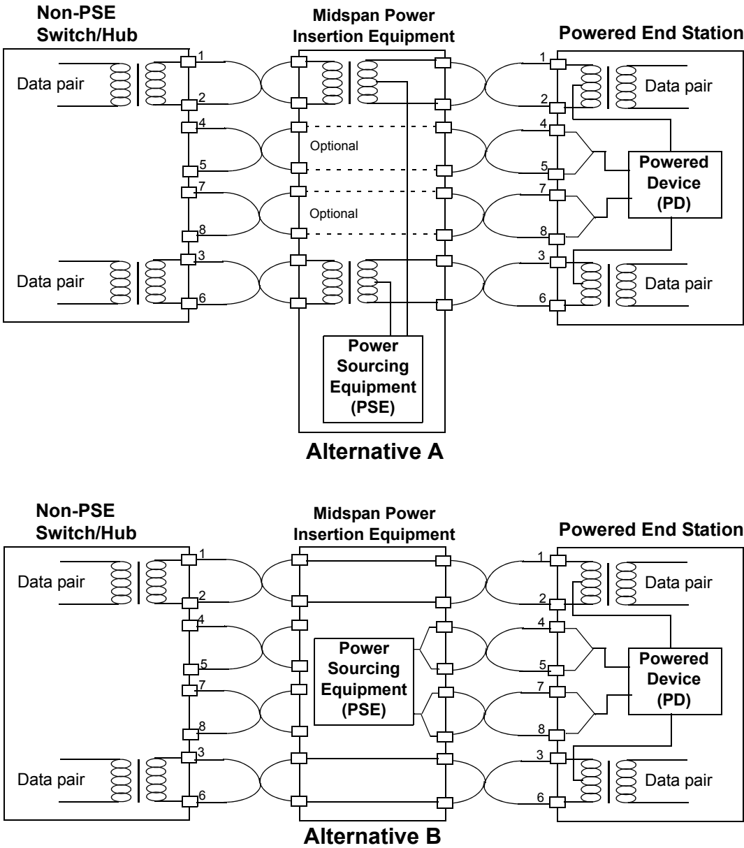
Figure 33-6—10BASE-T/100BASE-TX Midspan PSE location overview
