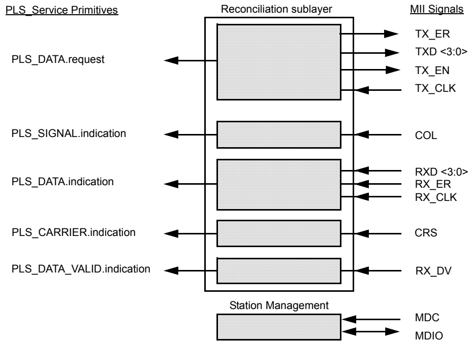
Figure 22–3 depicts a schematic view of the Reconciliation sublayer inputs and outputs, and demonstrates that the MII management interface is controlled by the station management entity (STA).
