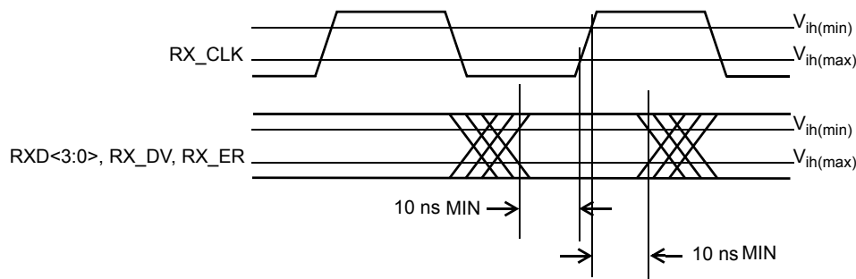
Figure 22-17—Receive signal timing relationships at the MII
