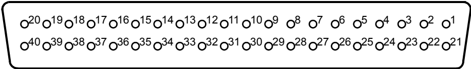
Figure 22–20—MII connector pin numbering
