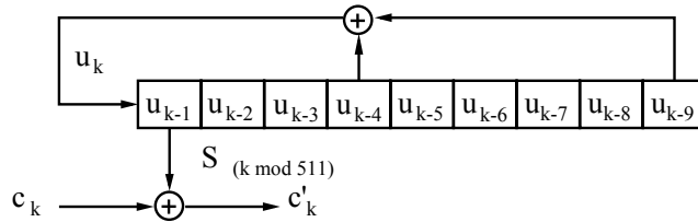
Figure 152—Chip whitening
