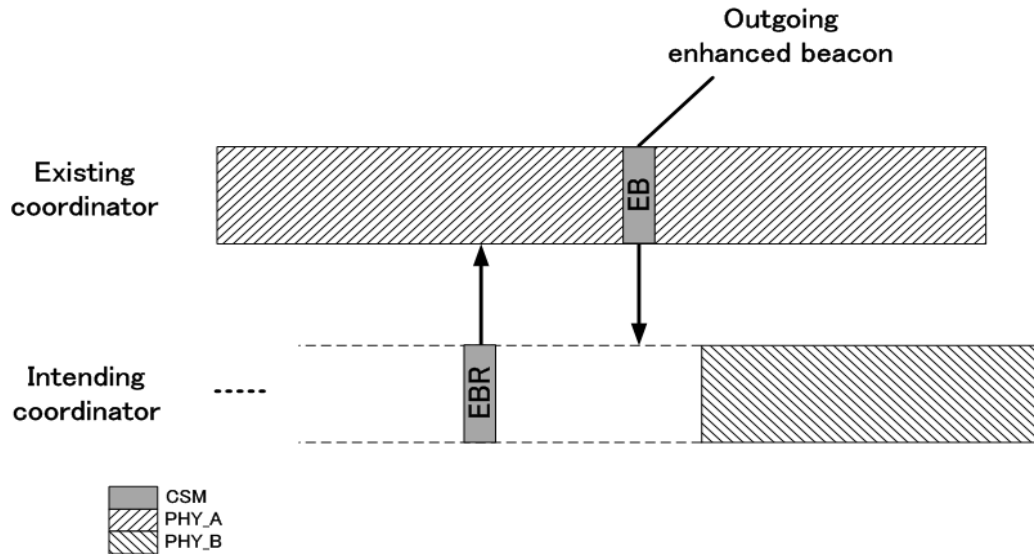
Figure 34w—Alternative method for inter-PHY mode coexistence in a nonbeacon-enabled PAN
