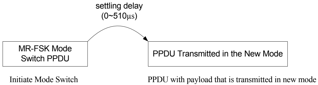
Figure 127—Transmitting sequence between MR-FSK mode switch PPDUs and the new mode PPDUs
