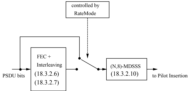
Figure 146—PSDU processing for MDSSS
