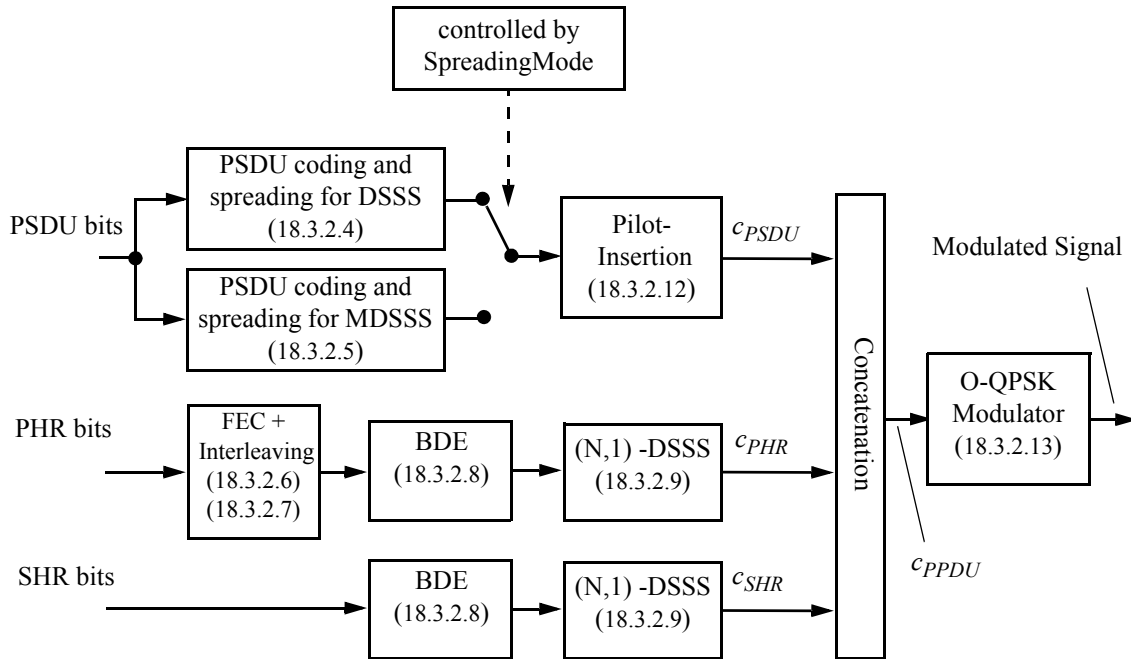
Figure 144—Reference modulator diagram
