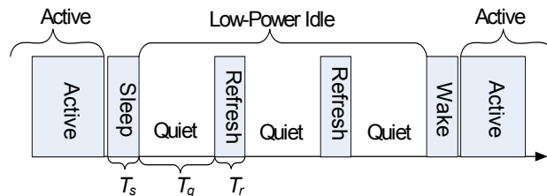
Figure 78–3—Overview of EEE LPI operation
