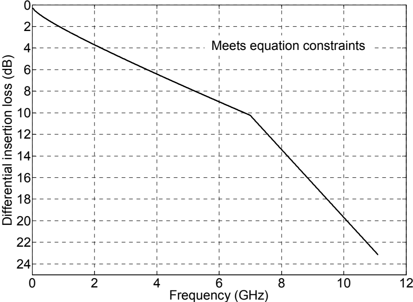
Figure 83B-1—Host insertion loss
