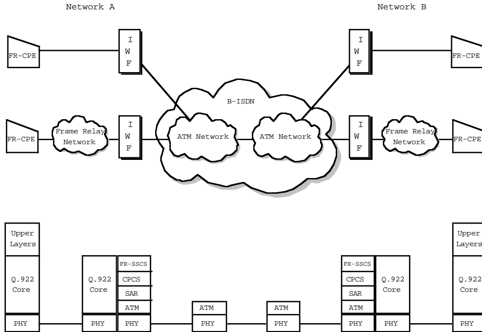
Figure 3: Network Interworking between FRBS and B-ISDN
