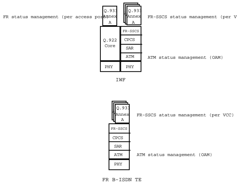
Figure 11: PVC Status Management Interworking Protocol Stack
