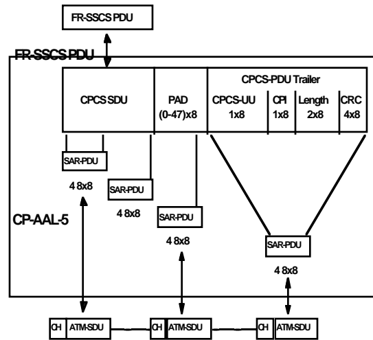
Figure 7: Common Part AAL-5 PDU Formats
