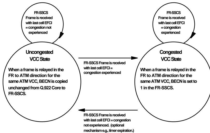
Figure 10: Congestion State Diagram for VCC
