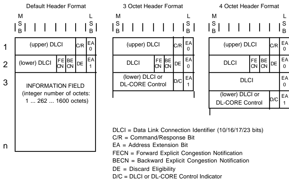
Figure 6: Structure of the FR-CS-PDU
