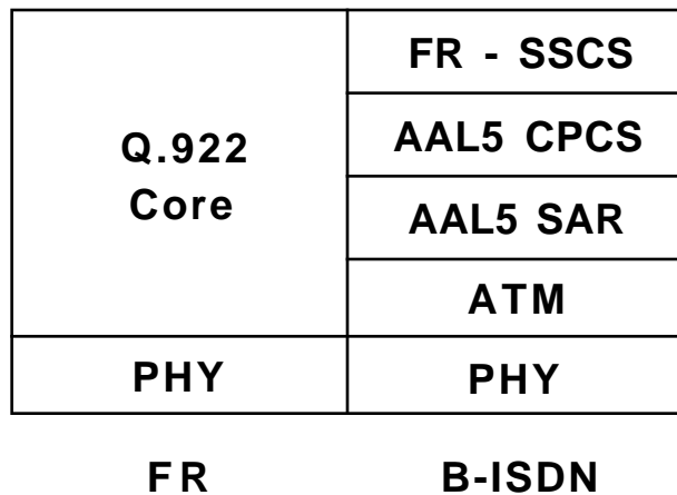
Figure 5: I.555 FR/ATM IWF Internal Architecture
