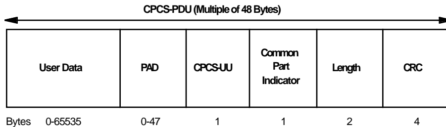
Figure 12: Format of the Common Part of the AAL Type 5 PDU (I.363)
