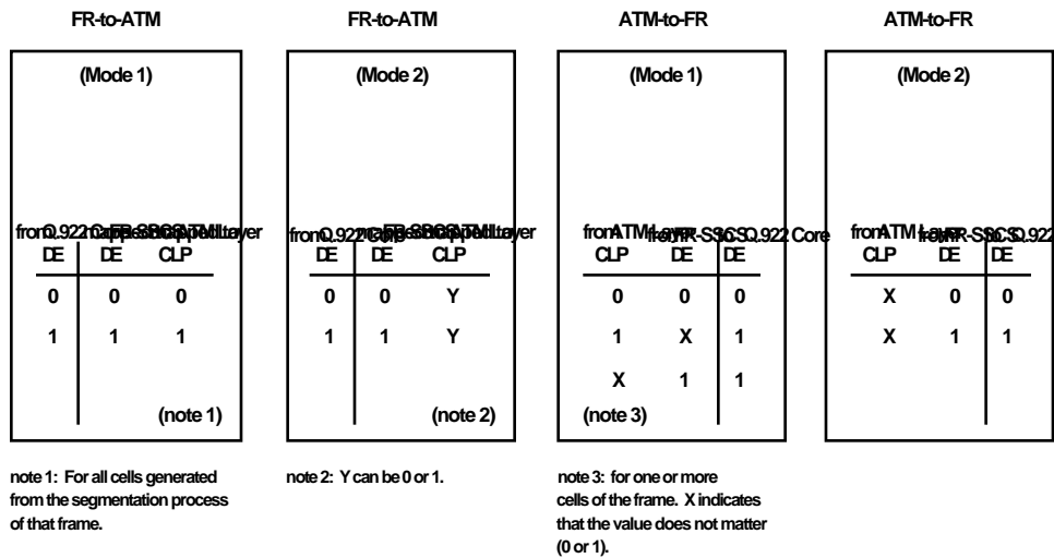
Figure 8: DE/CLP Mapping
