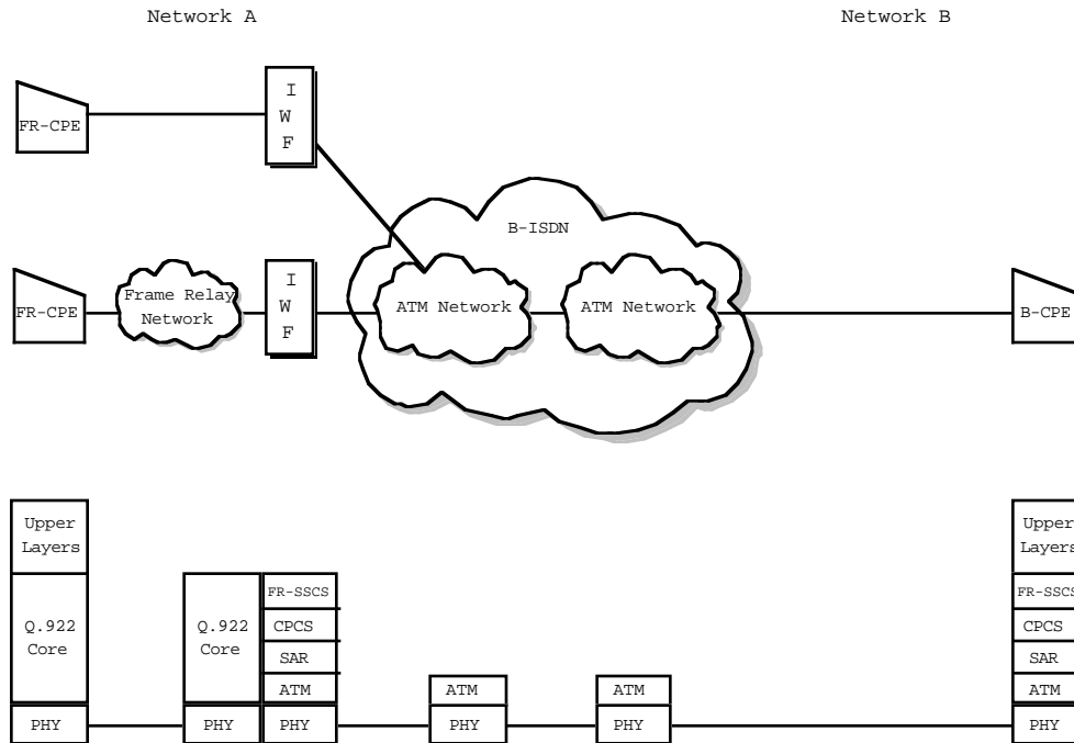
Figure 4: Network Interworking between FRBS and B-ISDN (I.555 Scenario 2)
