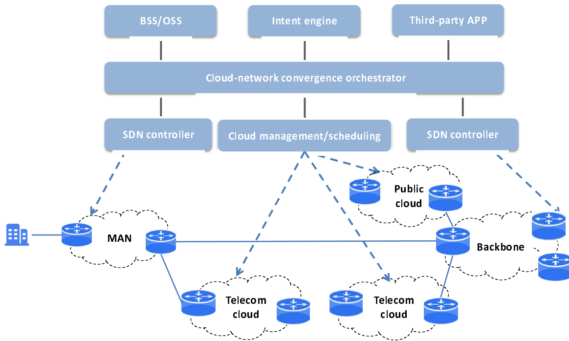
Figure 7: Architecture of Cloudified telecom network
