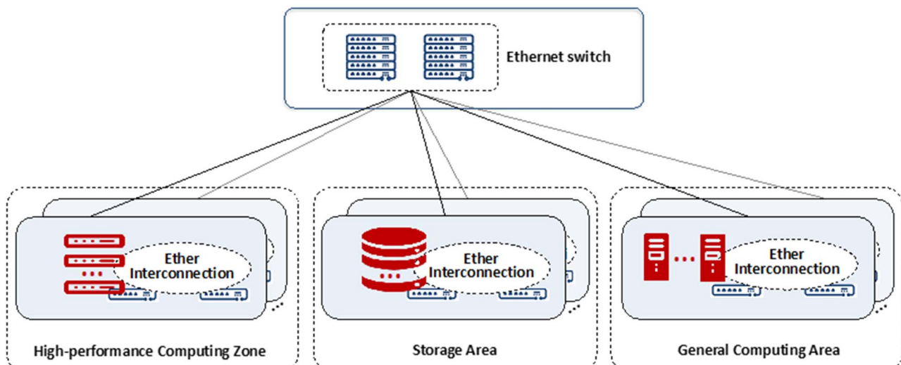
Figure 12: Architecture of the lossless Ethernet networking
