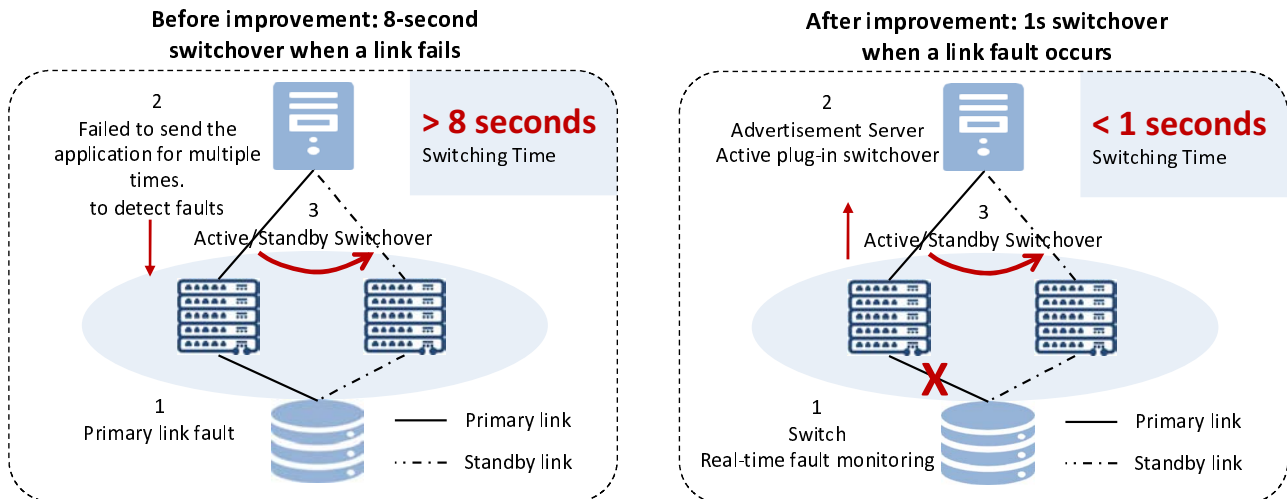
Figure 10: Improvement in fault recovery time
