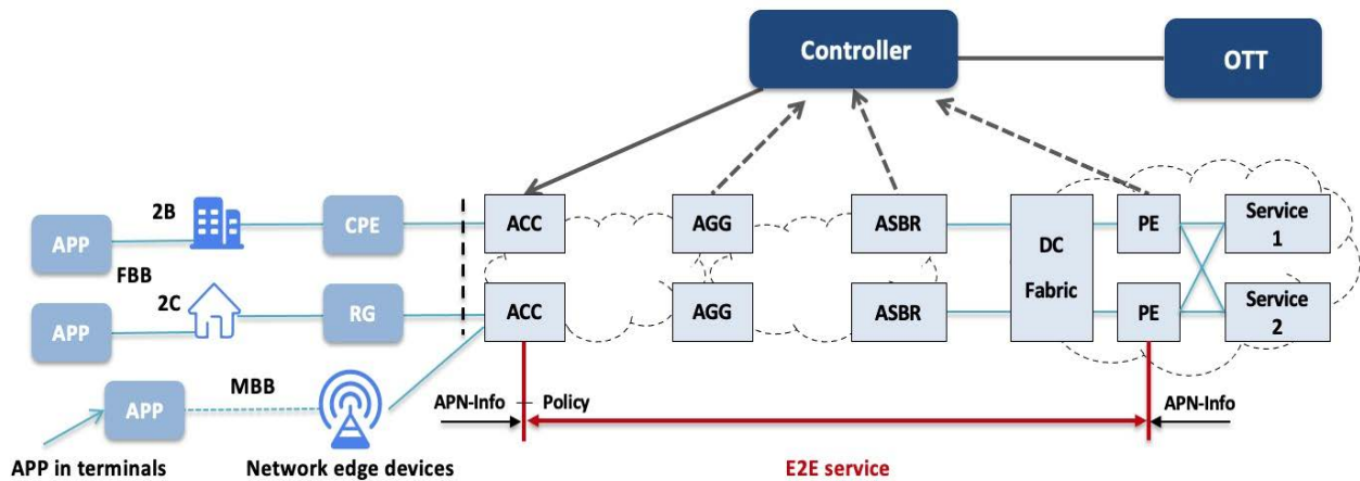
Figure 3: Connections of Enterprise Site to DCs
