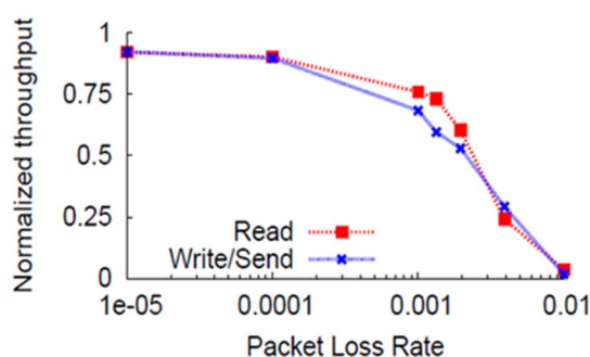
Figure 8: Impact of network packet loss on throughput
