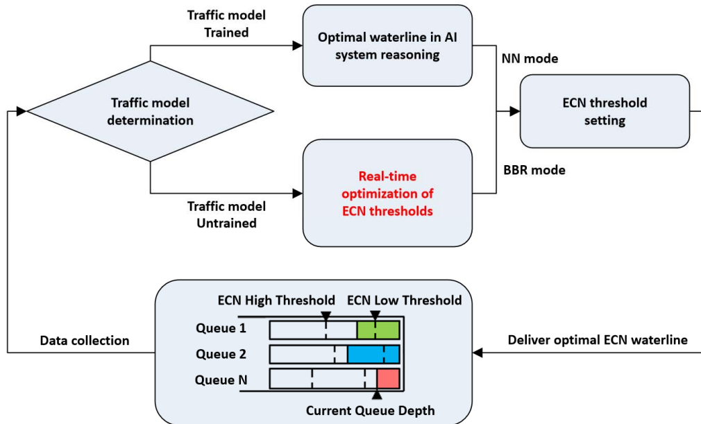
Figure 9: AI Explicit Congestion Notification Algorithm Framework
