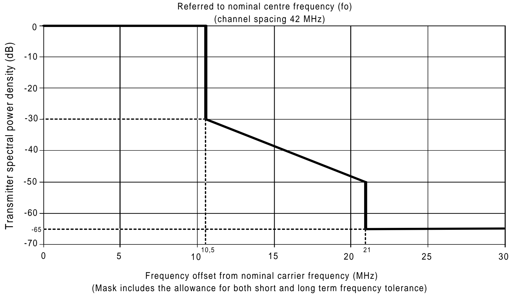
Figure 8: Limits of spectral power density for video basebands up to 3,5 MHz
