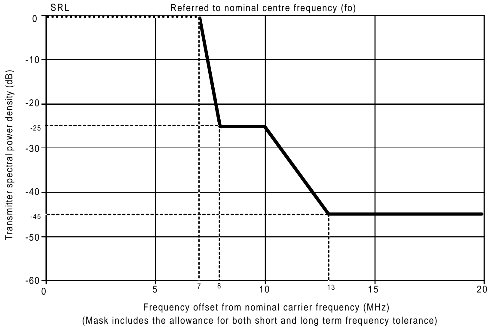
Figure 3: Limits of spectral power density for minimum system rate of 2 Mbit/s using channel spacing of 14 MHz
