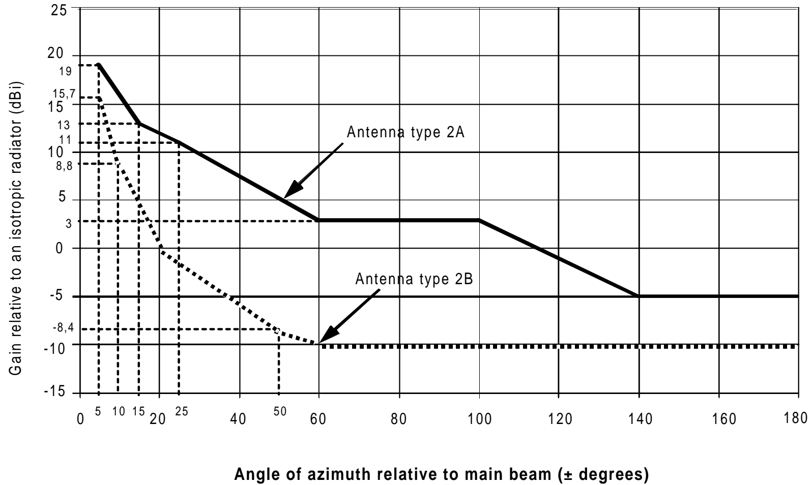
Figure 2: Limits of antenna gain for angles greater than 5° from the main beam axis
