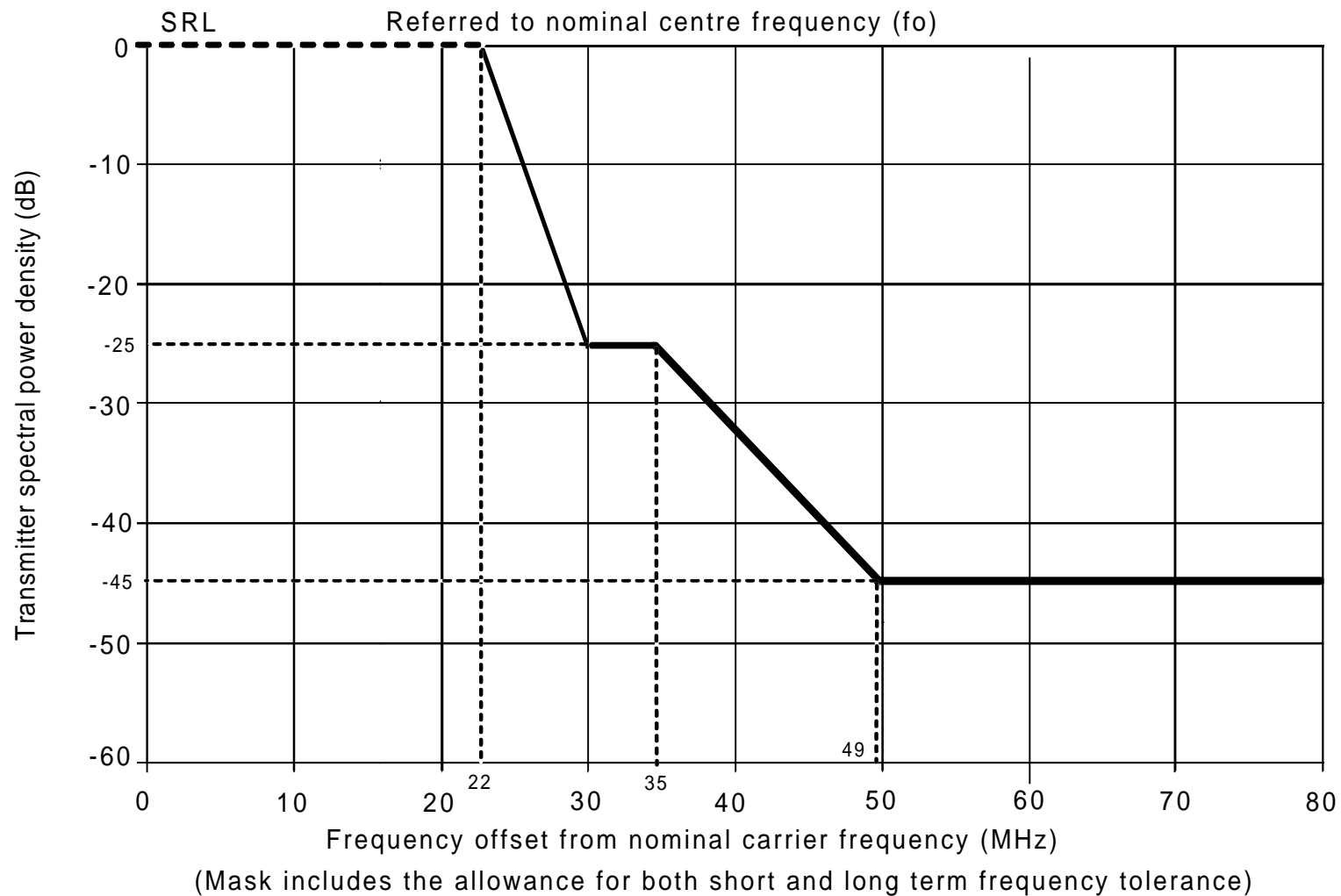
Figure 5: Limits of spectral power density for minimum system rate of 34 Mbit/s using channel spacing of 56 MHz
