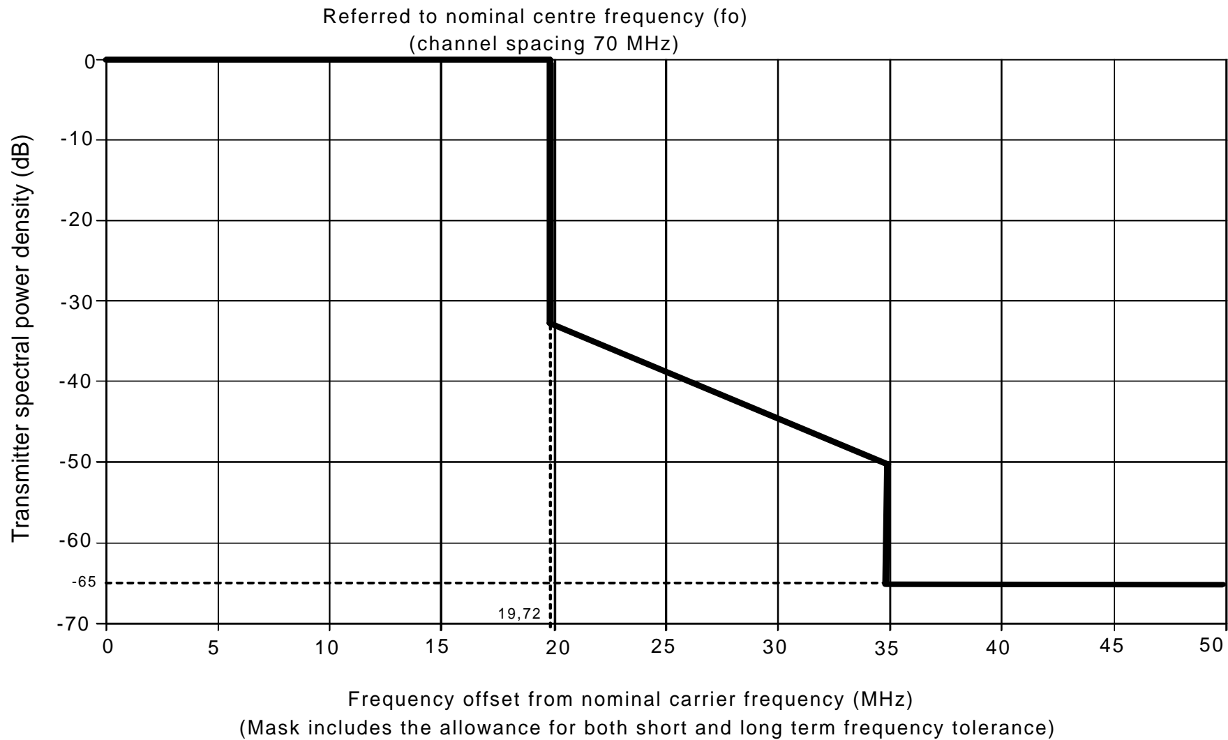
Figure 9: Limits of spectral power density for video basebands up to 14 MHz
