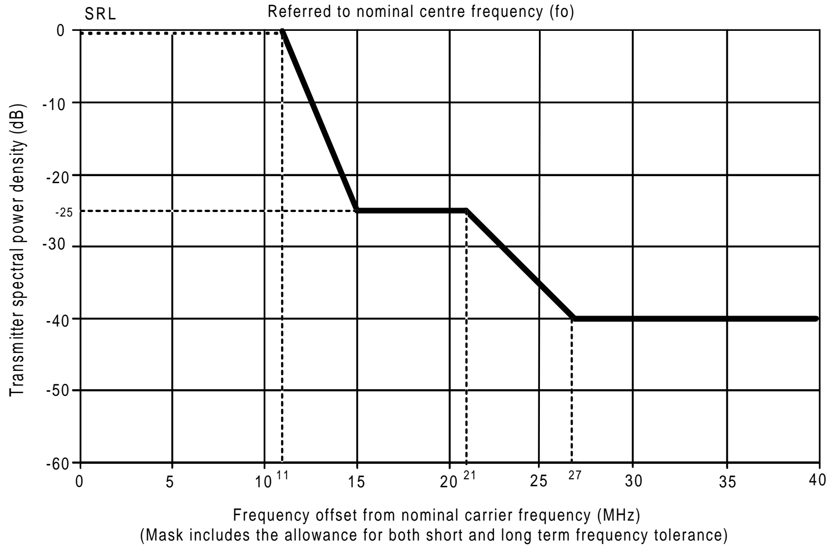
Figure 4: Limits of spectral power density for minimum system rate of 8 Mbit/s using channel spacing of 28 MHz
