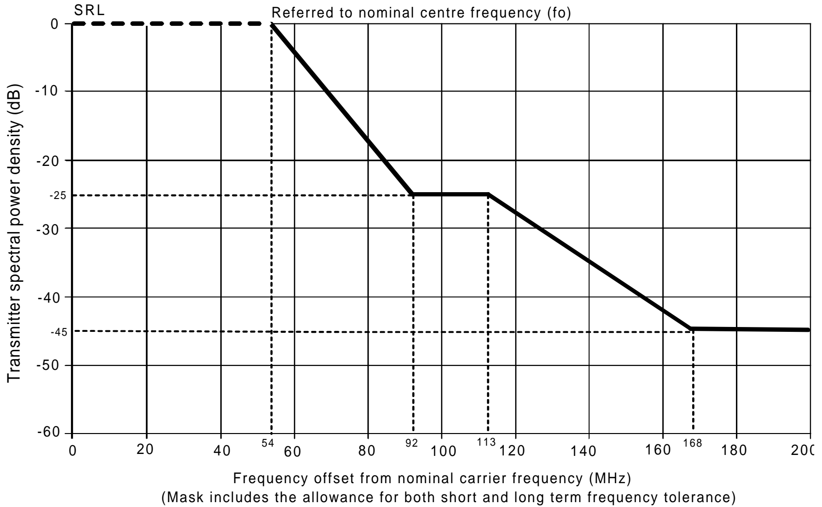
Figure 6: Limits of spectral power density for minimum system rate of 140/155 Mbit/s using channel spacing of 140 MHz
