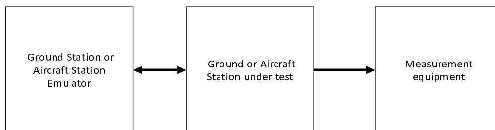
Figure B.1: Measurement system for transmitter spurious emissions
