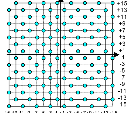
Figure 6-20: Symbol Constellations
