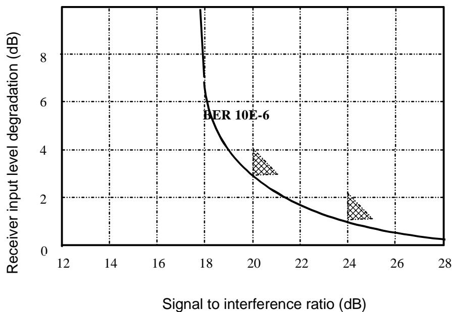
Figure 5: Co-channel "internal" digital interference sensitivity limits referred to point B'
