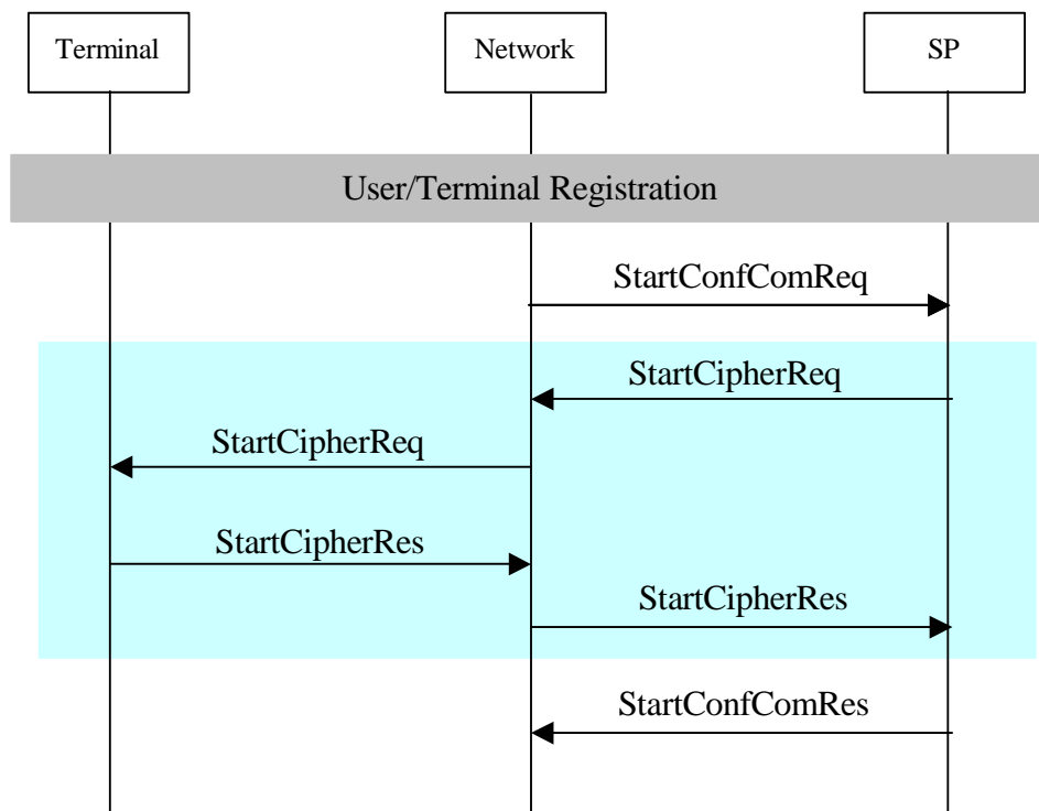
Figure 25: Information flow for user update of profile held by their Service Provider
