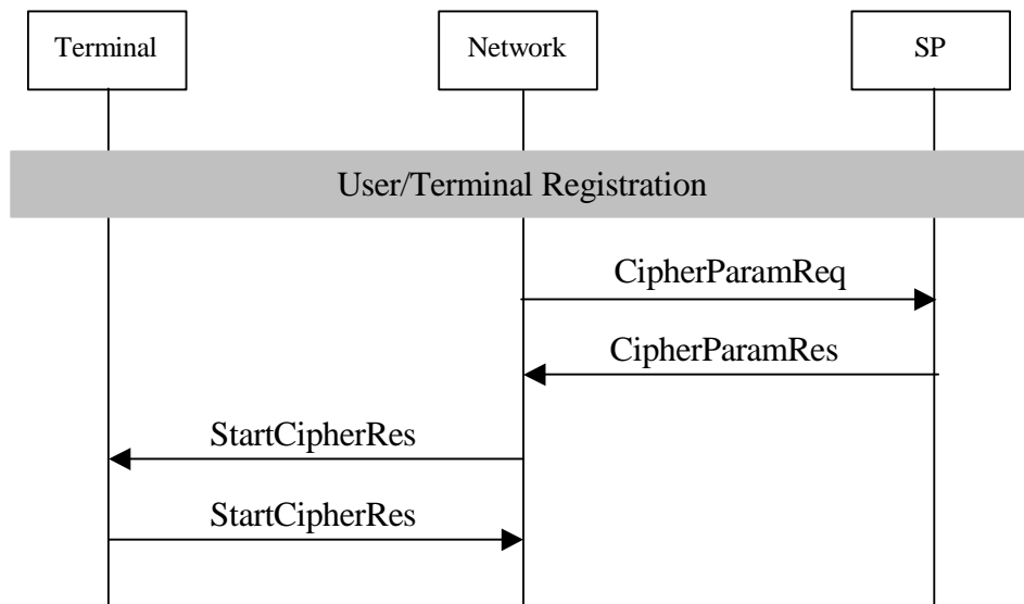
Figure 24: Information flow for network initiated confidential communication mode
