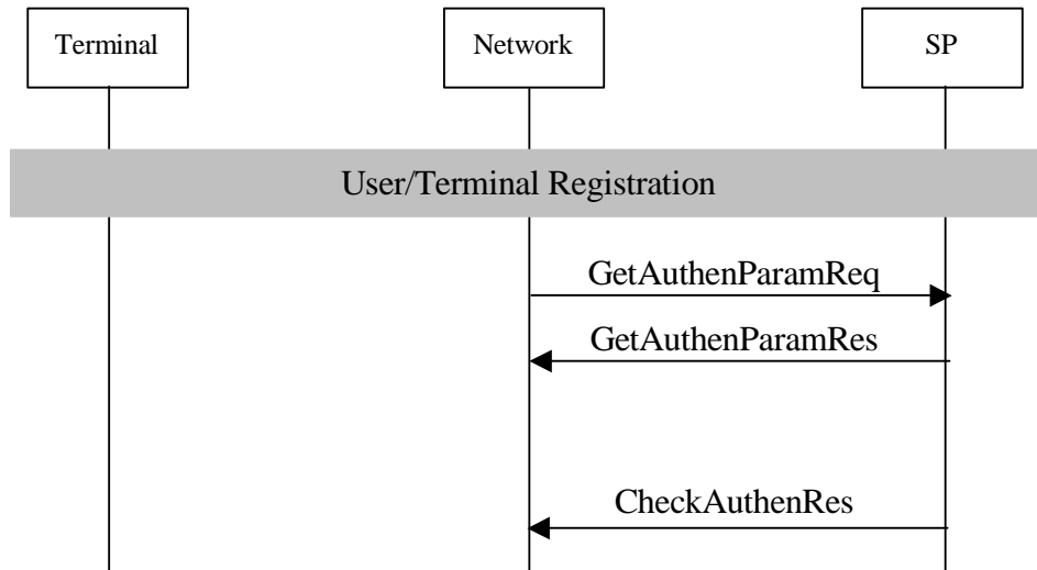
Figure 32: Information flow for the PTN request for authentication of the SP served user
