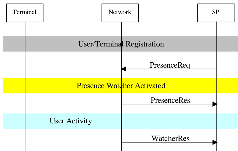
Figure 39: Information flow for Service Provider request the presence operation
