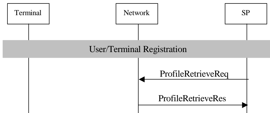
Figure 13: Information flow for SP retrieval of profile from the PTN
