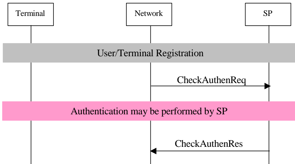
Figure 31: Information flow for the PTN request for authentication of the SP served user
