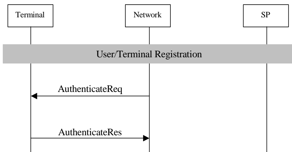
Figure 33: Information flow for the PTN performing terminal authentication
