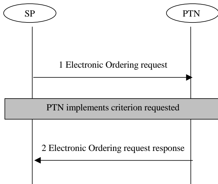
Figure 29: Electronic ordering of network management functions
