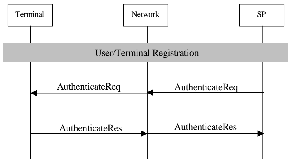
Figure 30: Information flow for Service Provider request for user authentication
