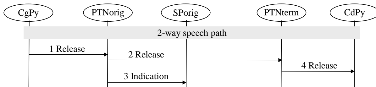
Figure 14a: Scenario where SPorig is notified about the CdPy disconnecting the call
