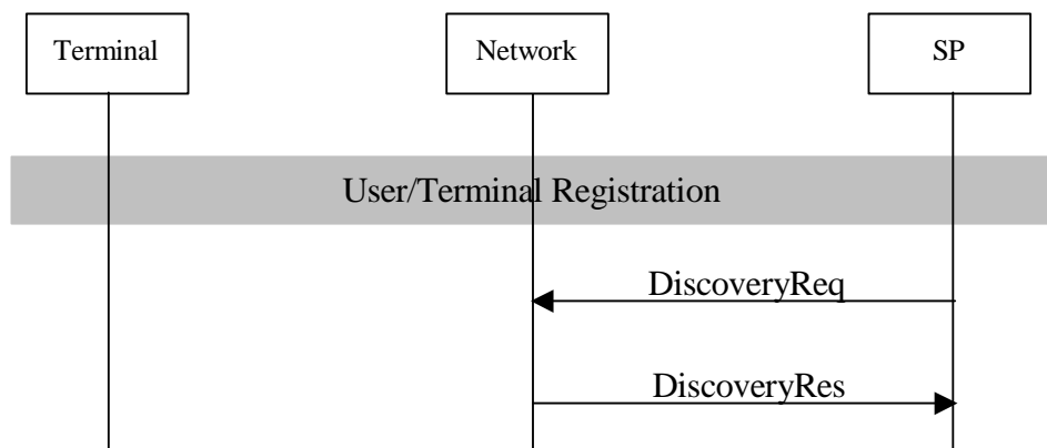
Figure 37: Information flow for Service Provider request the discovery operation
