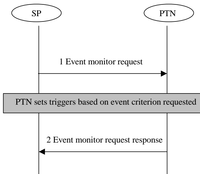
Figure 28: Request for event monitoring and subsequent reporting
