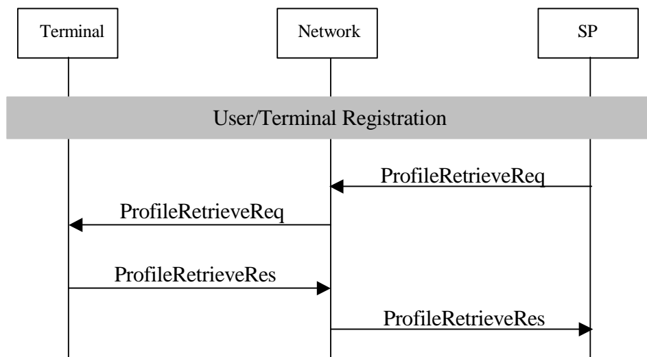
Figure 8: Information flow for SP retrieval of profile from their service user's terminal
