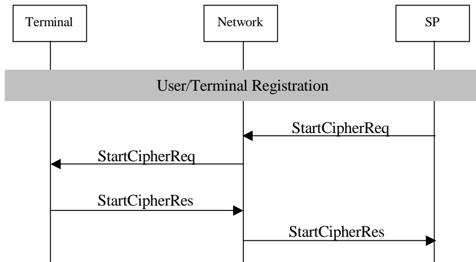
Figure 23: Information flow for SP requesting the start confidential communications
