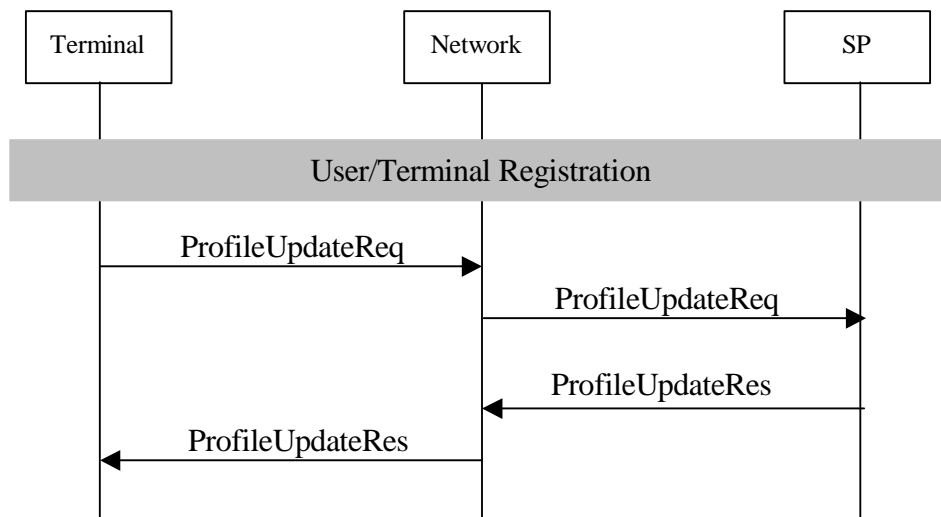
Figure 11: Information flow for user update of profile held by their Service Provider
