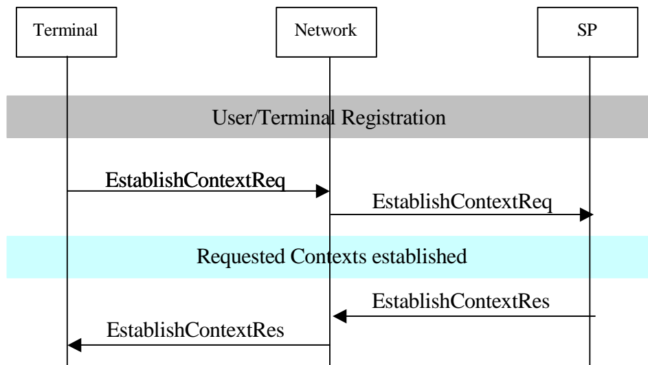
Figure 36: Information flow for Service Provider request the discovery operation
