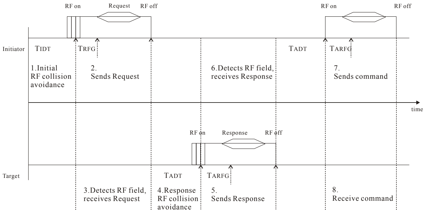
Figure 22 – Initialisation flow for Active communication mode
