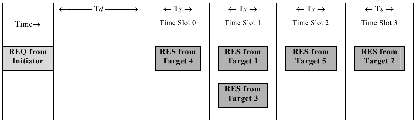
Figure 19 – Single Device Detection by Time Slot
