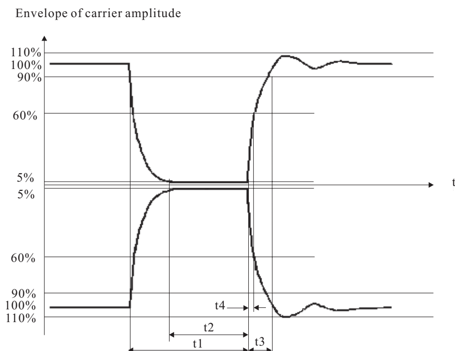
Figure 1 – Pulse shape
