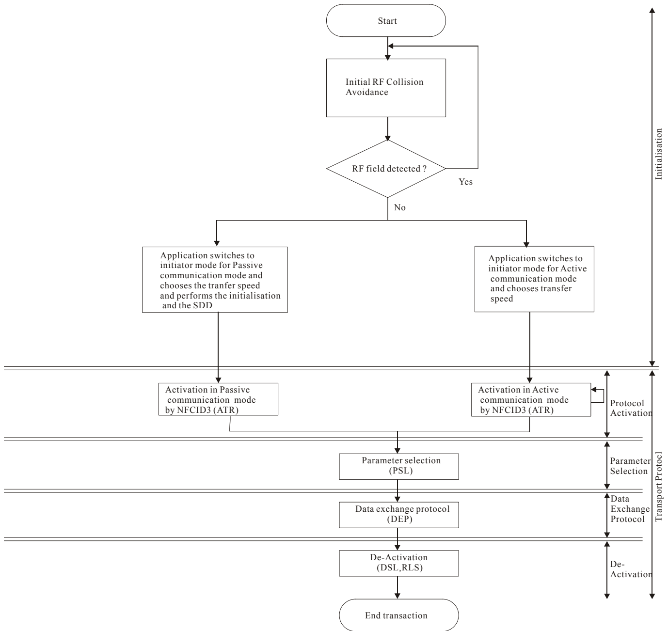
Figure 5 – General initialisation and single device detection flow
