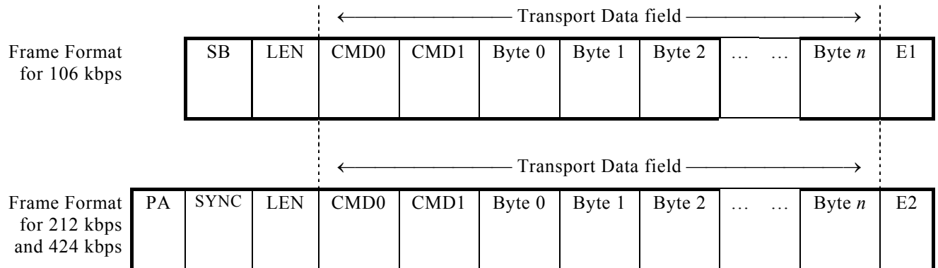
Figure 23 – Transport Frame format Definition
