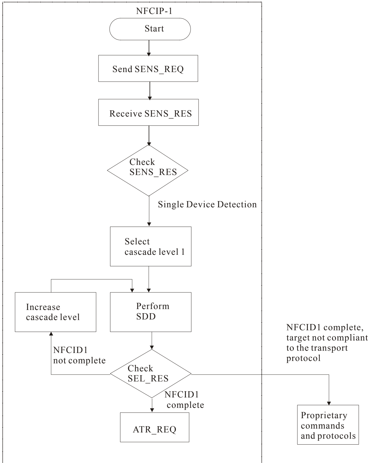
Figure 13 – Initialisation and SDD Flow Chart for Initiator
