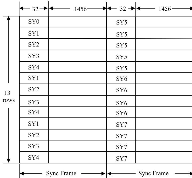
Figure 23 - Physical Sector
