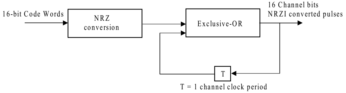
Figure 22 - NRZI conversion
