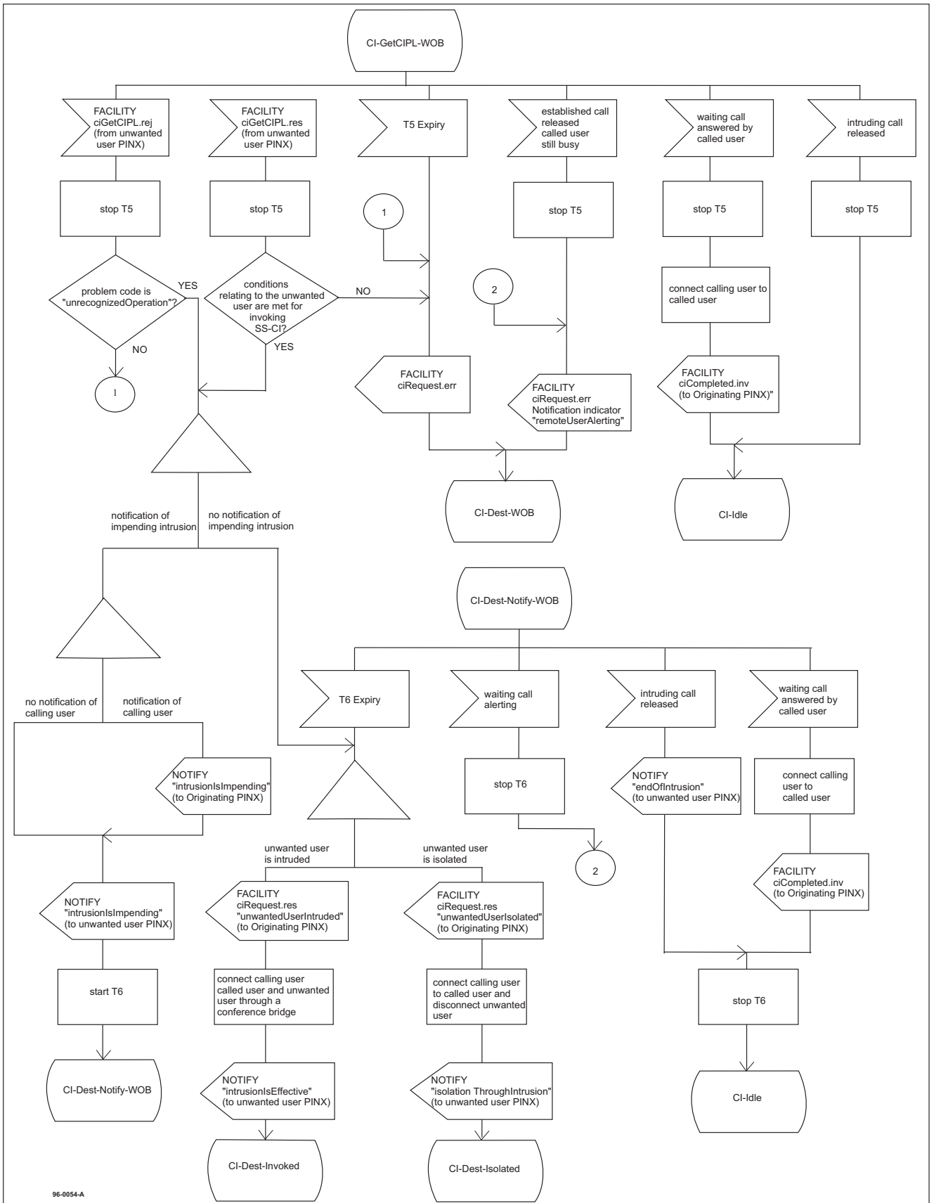
Figure D.2 (sheet 6 of 6) - Terminating PINX SDL
