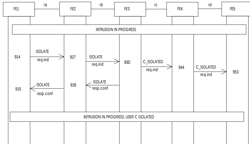
Figure 11 - Information flow sequence - normal operation of SS-CI, normal operation, isolation of user C
