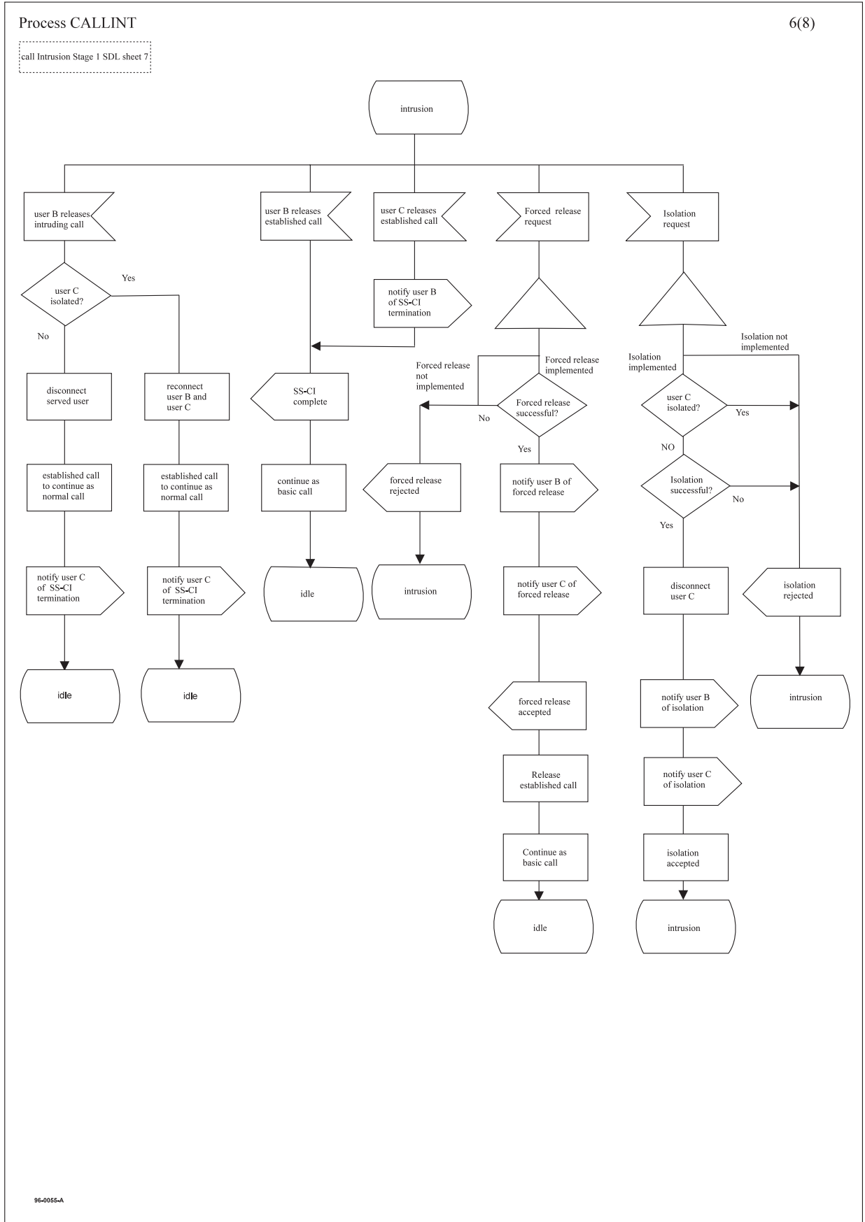
Figure 1 - SS-CI, overall SDL (part 6 of 8)
