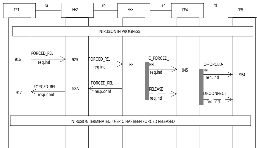
Figure 12 - Information flow sequence - normal operation of SS-CI, normal operation, forced release of user C
