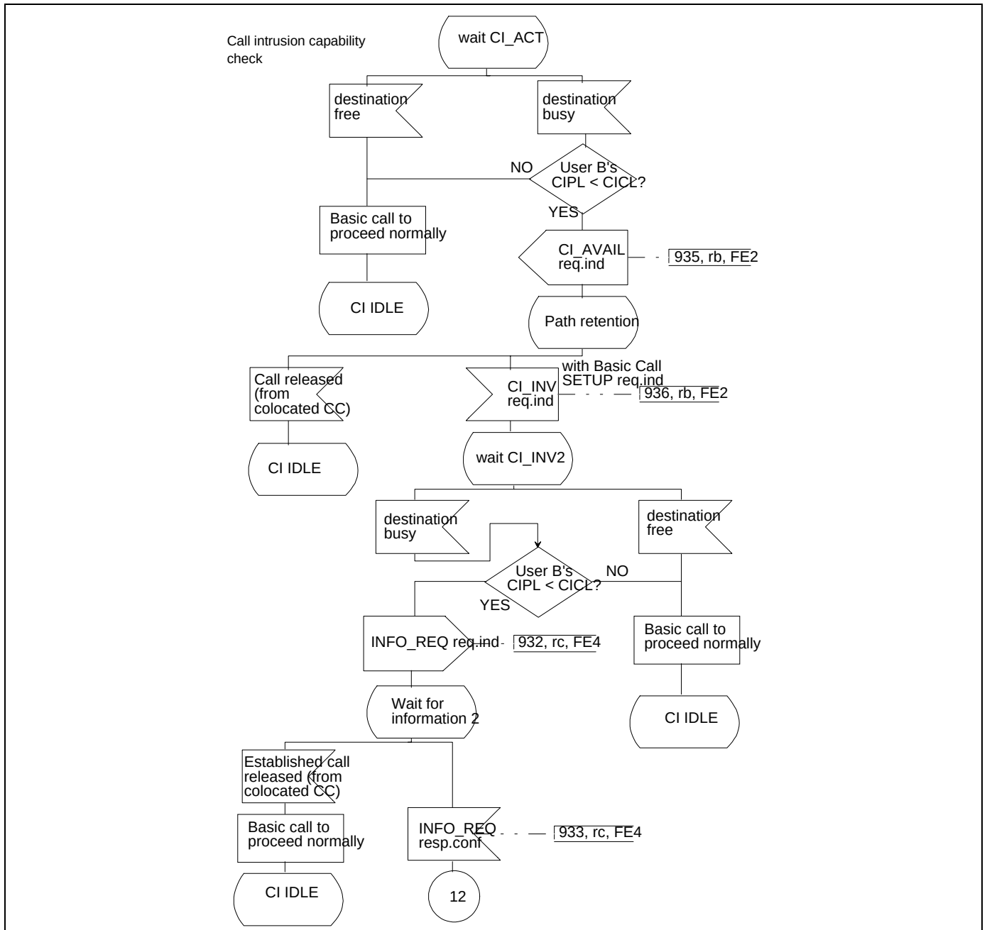
Figure 19 - SS-CI, SDL for functional entity FE3 (part 2 of 8)
