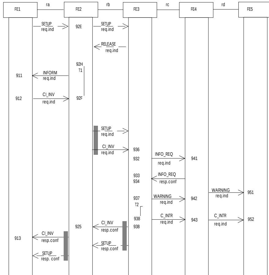
Figure 5 - Information flow sequence - normal operation of SS-CI, normal operation, consultation, non-retention
