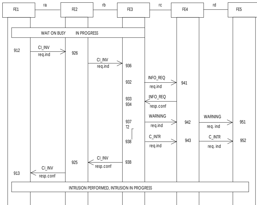
Figure 16 - Information flow sequence - normal operation of SS-CI, normal operation, new intrusion during the wait on busy state is requested
