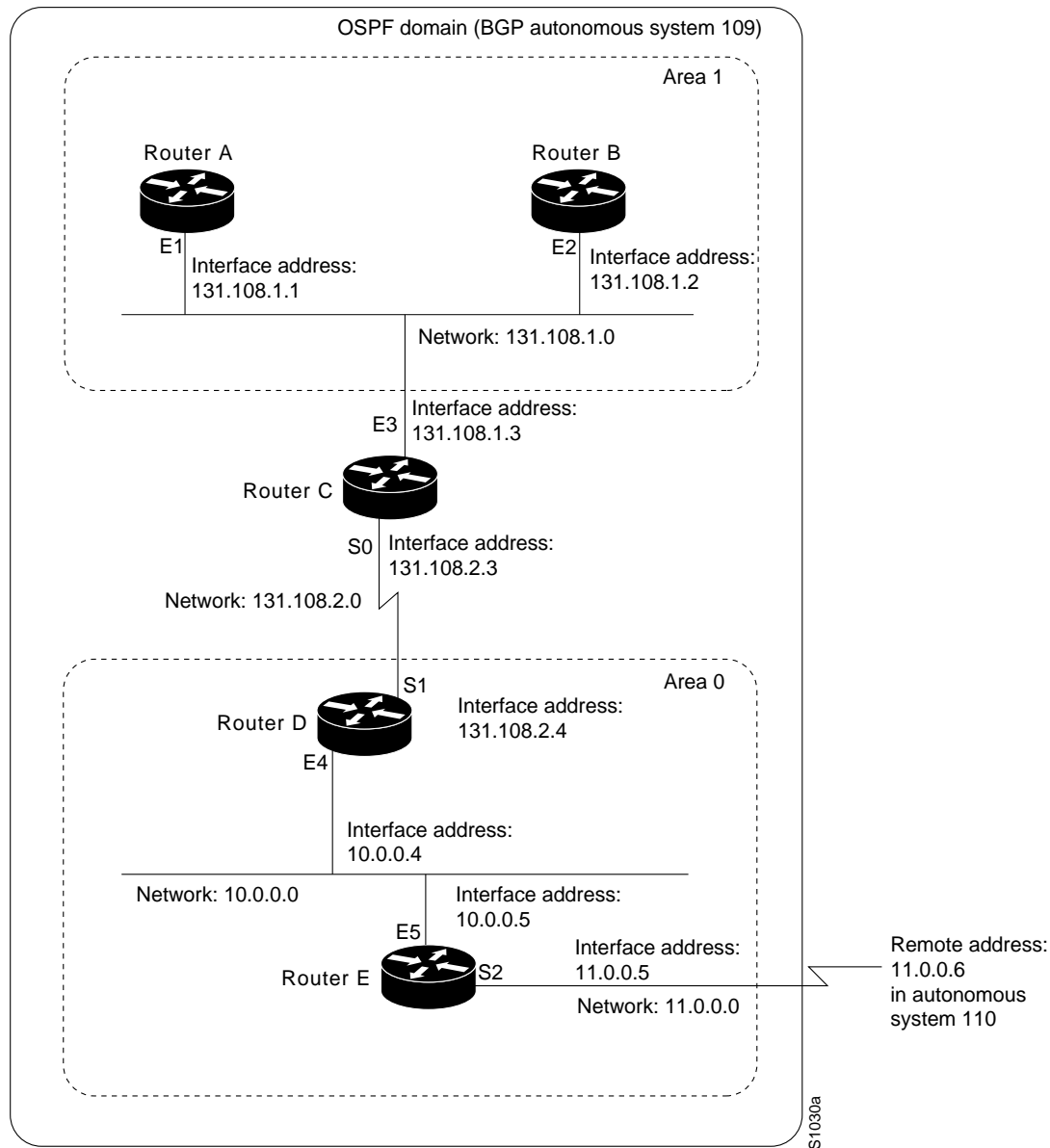
Figure 61 Example OSPF Autonomous System Network Map
