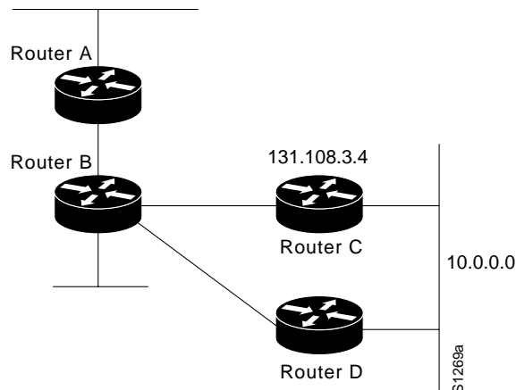
Figure 60 Overriding Static Routes
