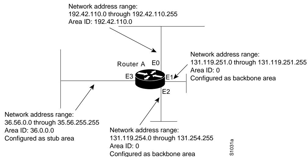
Figure 62 Interface and Area Specifications for OSPF Configuration Example
