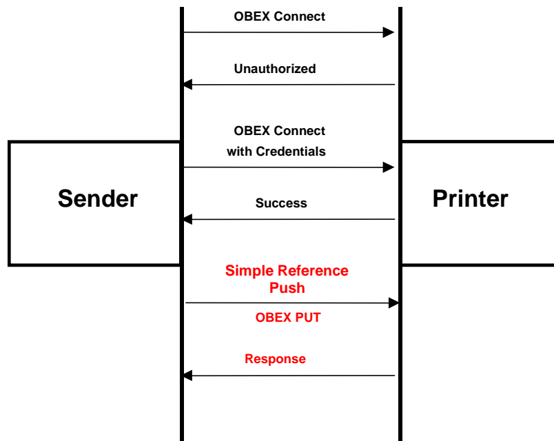
Figure 8.4: Printer Access Control
