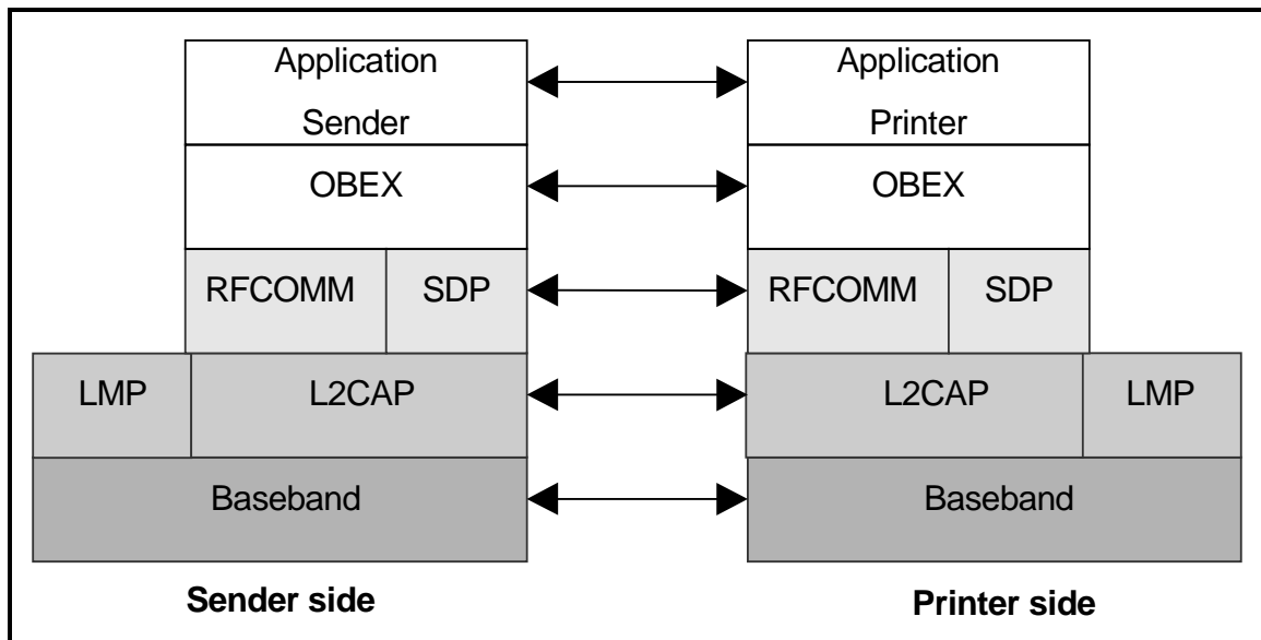
Figure 2.1: Protocol Model
