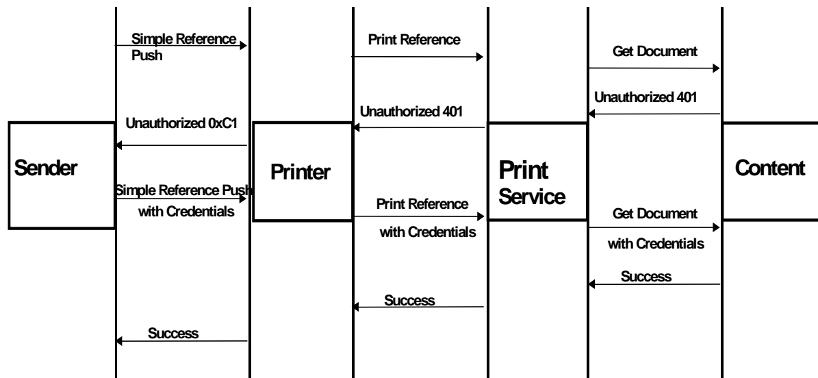
Figure 8.6: Security Challenge with Print Service
