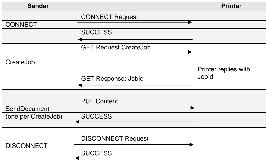
Figure 11.1: Session Signaling Diagram
