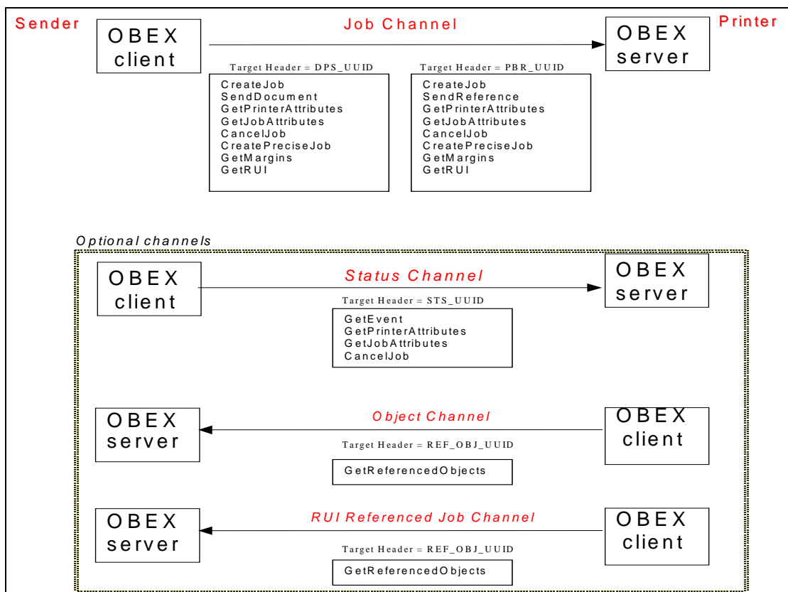
Figure 5.2: Job-Based Transfer Model Connections
