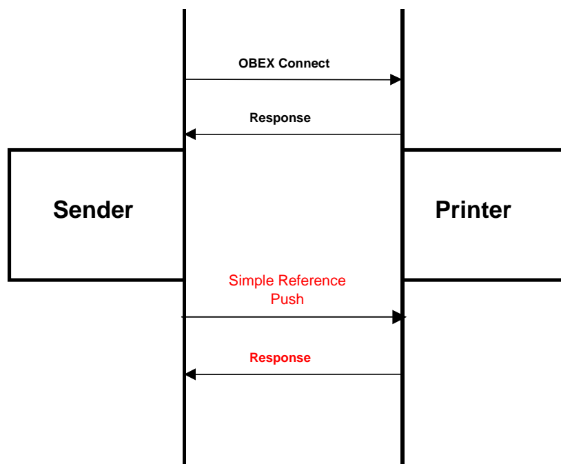
Figure 8.3: Reference Transfer
