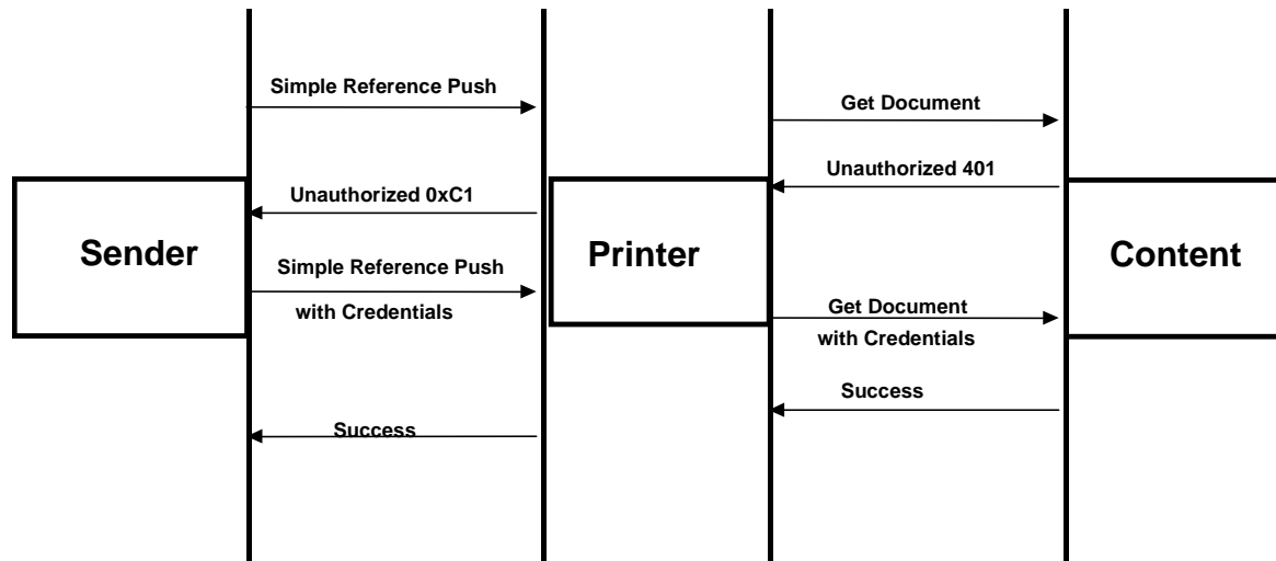
Figure 8.5: Security Challenge
