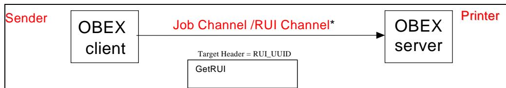
Figure 5.3: Printer Administration RUI Connections
