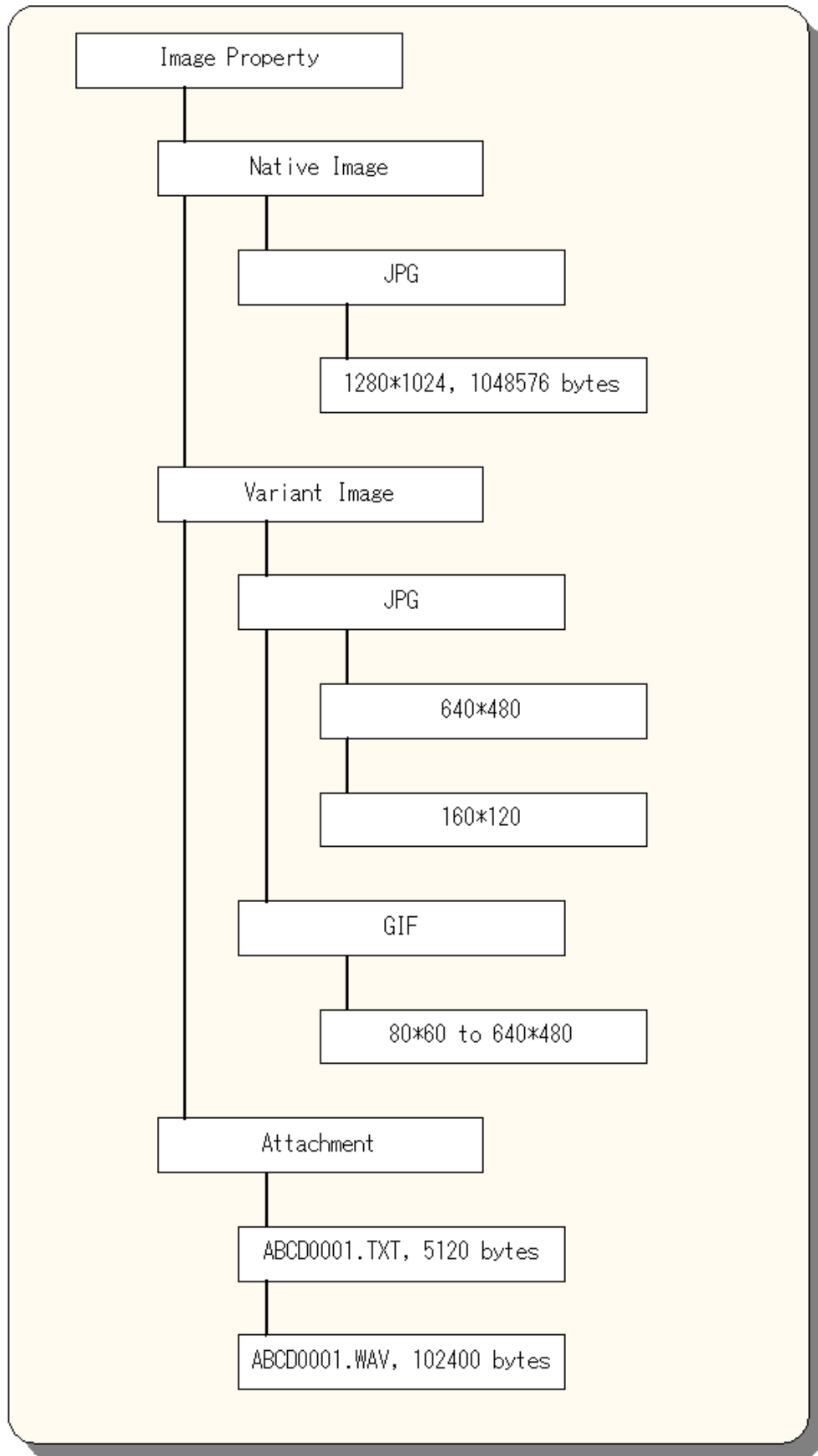
Figure 4-8: Example image-properties Representation
