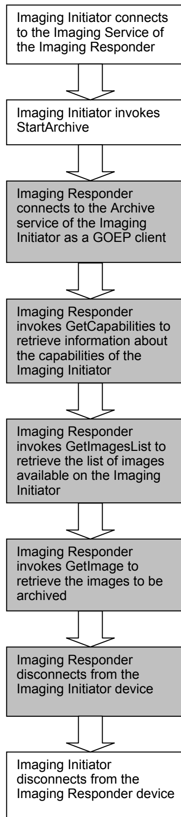
Figure 4-5: Typical Automatic Archive Sequence
