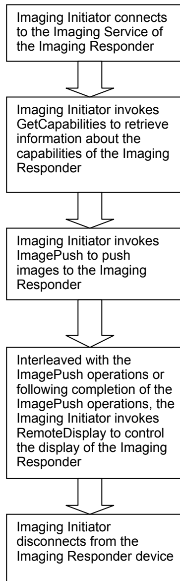
Figure 4-7: Typical Remote Display Sequence
