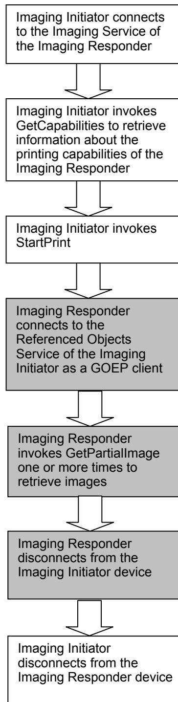
Figure 4-4: Typical Advanced Image Printing Sequence
