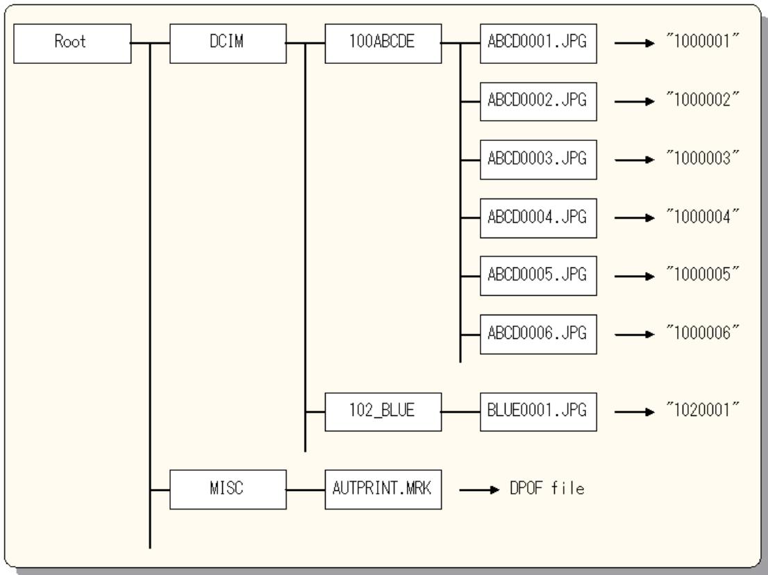
Figure 4-9: Example File System Structure
