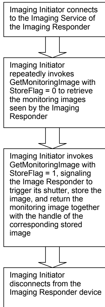
Figure 4-6: Typical Remote Camera Sequence
