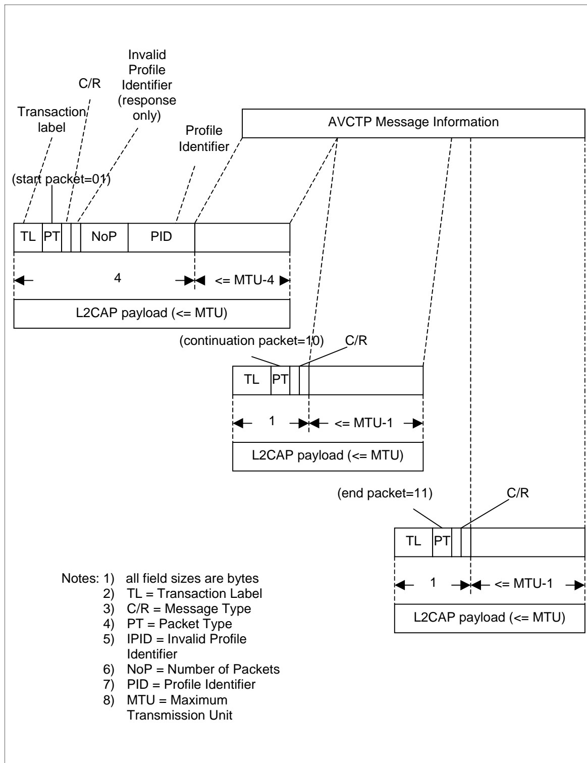
Figure 6.2: Fragmented AVCTP Message: Encapsulation
