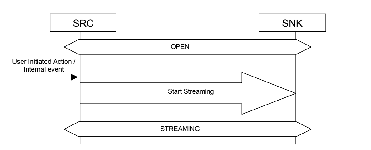
Figure 13.2: Audio Streaming
