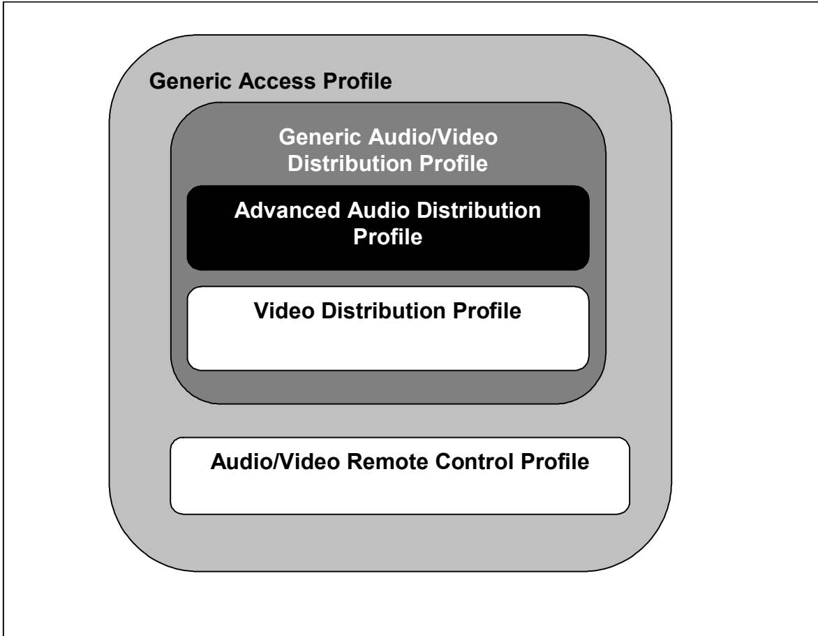
Figure 1.1: Profile Dependencies
